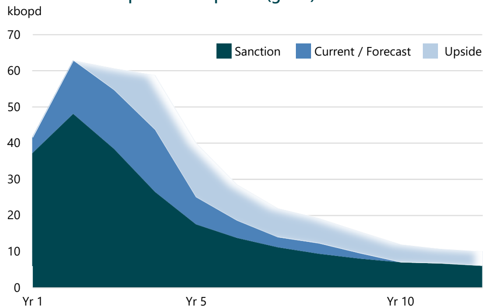
Catcher Area oil production profile (gross)
