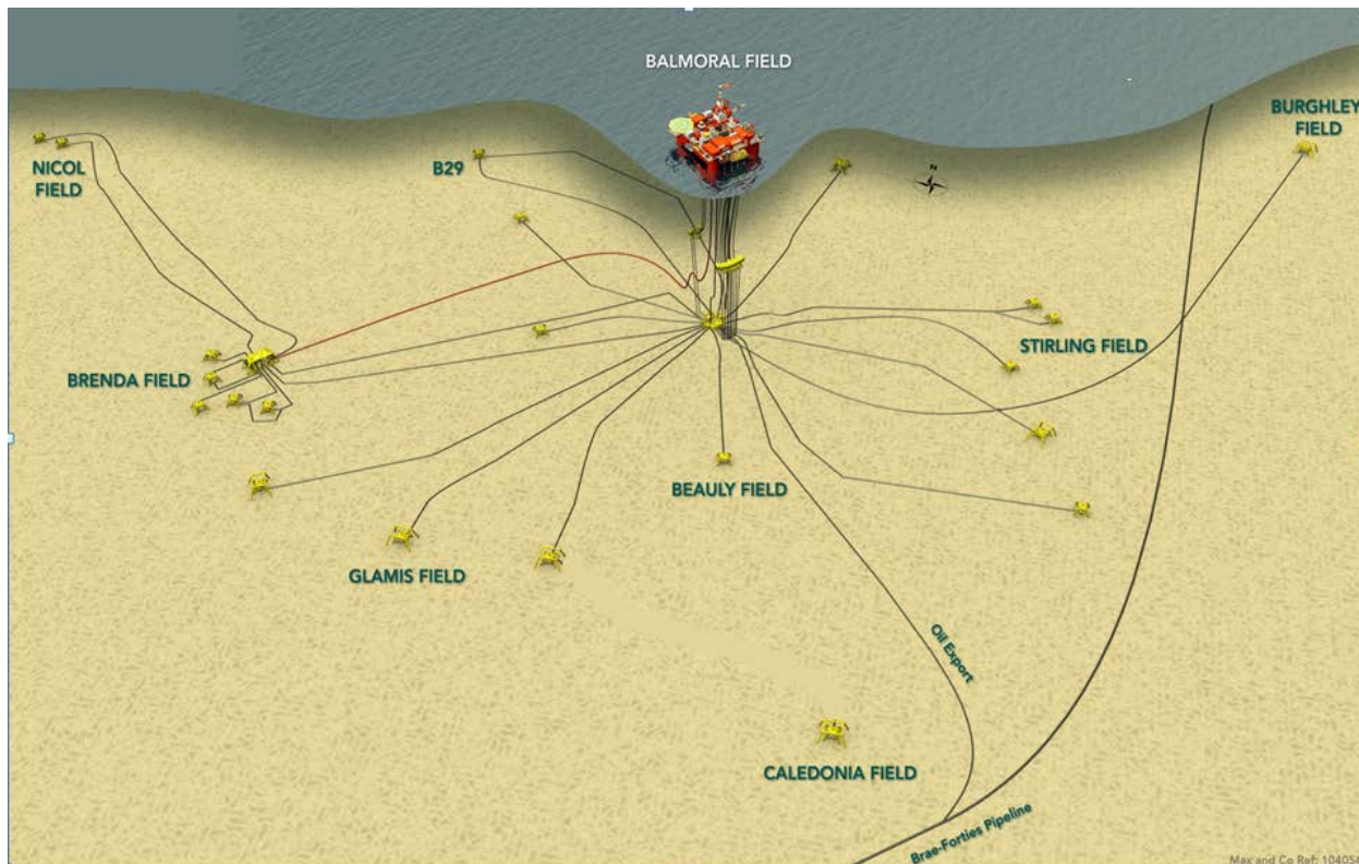
Figure 1.2: Field Layouts
