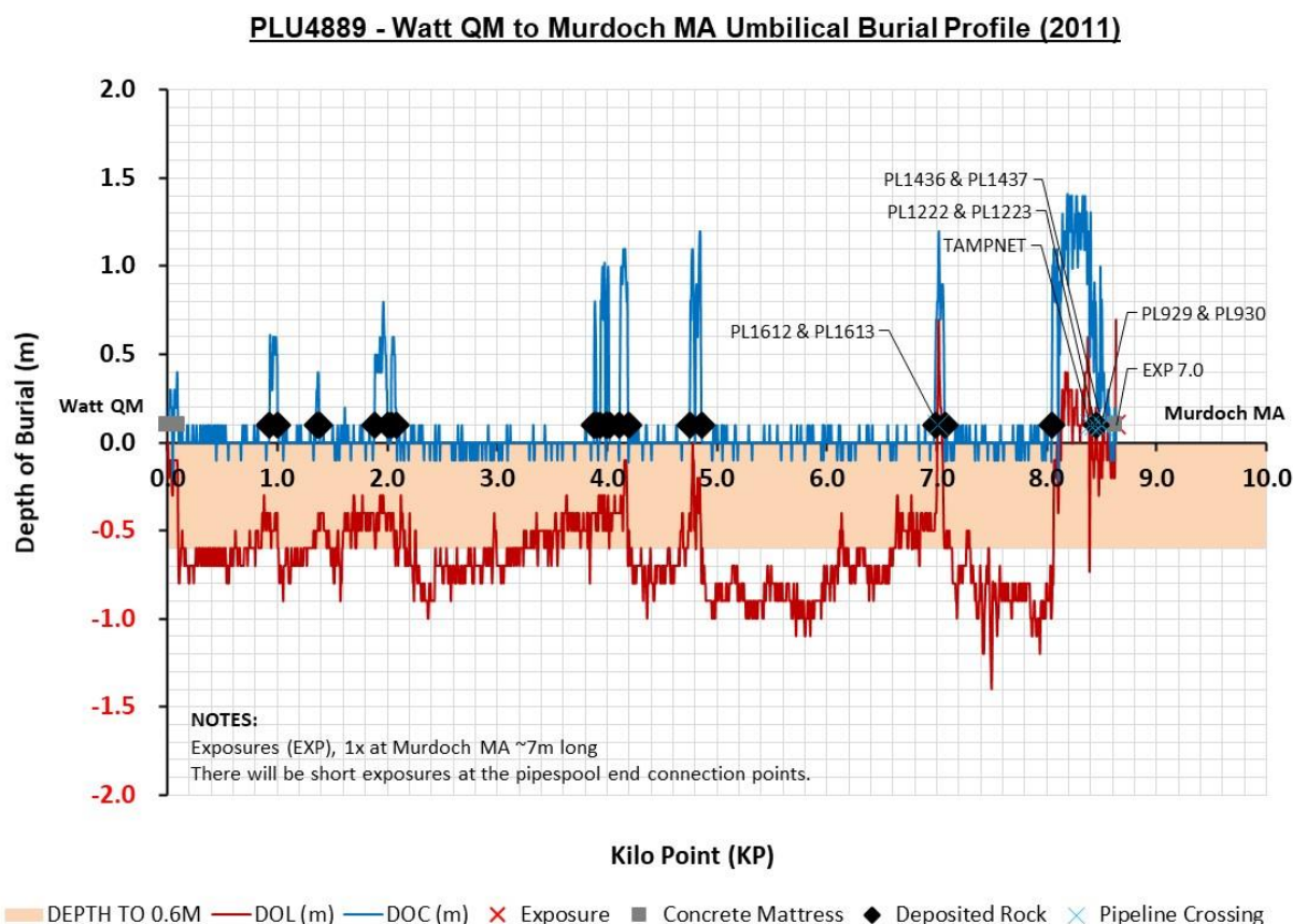
Figure 3.12.3: PLU4889 depth of cover profile ~KP-0.0 to ~KP8.64 (2011)
