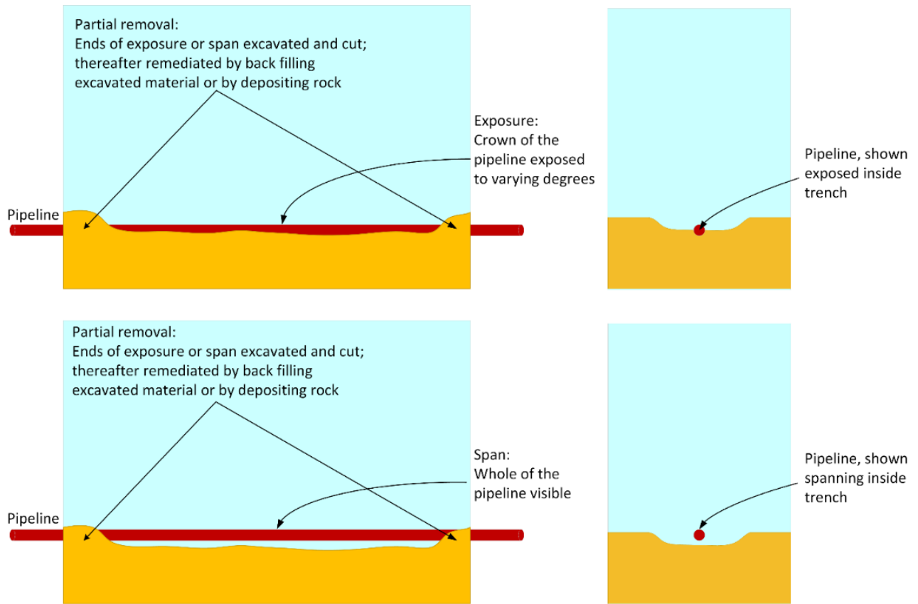
Figure 4.2.1: Exposures, spans & partial removal
