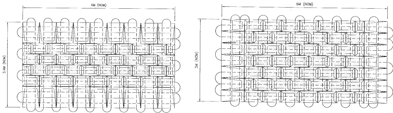
Figure 2.4.6: Fronded mattresses Type 6m x 3.4m x 0.3m & 6m x 3m x 0.15m
