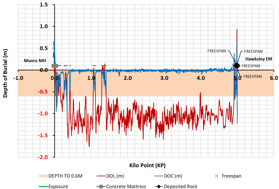
Figure 3.8.3: PL2109 & PL2110 depth of cover profile ~KP-0.05 to ~KP16.98 (2009/17)
