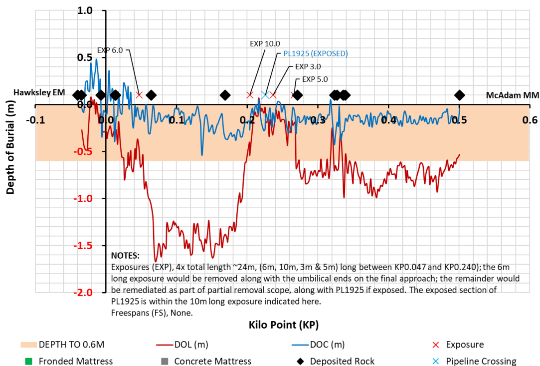
Figure 3.11.4: PLU4685 depth of cover profile ~KP-0.04 to ~KP0.50 (2007)
