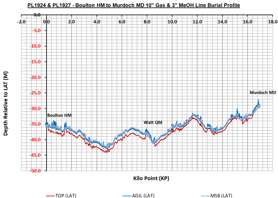
Figure 3.7.1: PL1924 & PL1927 seabed & burial profile ~KP-0.05 to ~KP16.98 (2009)
