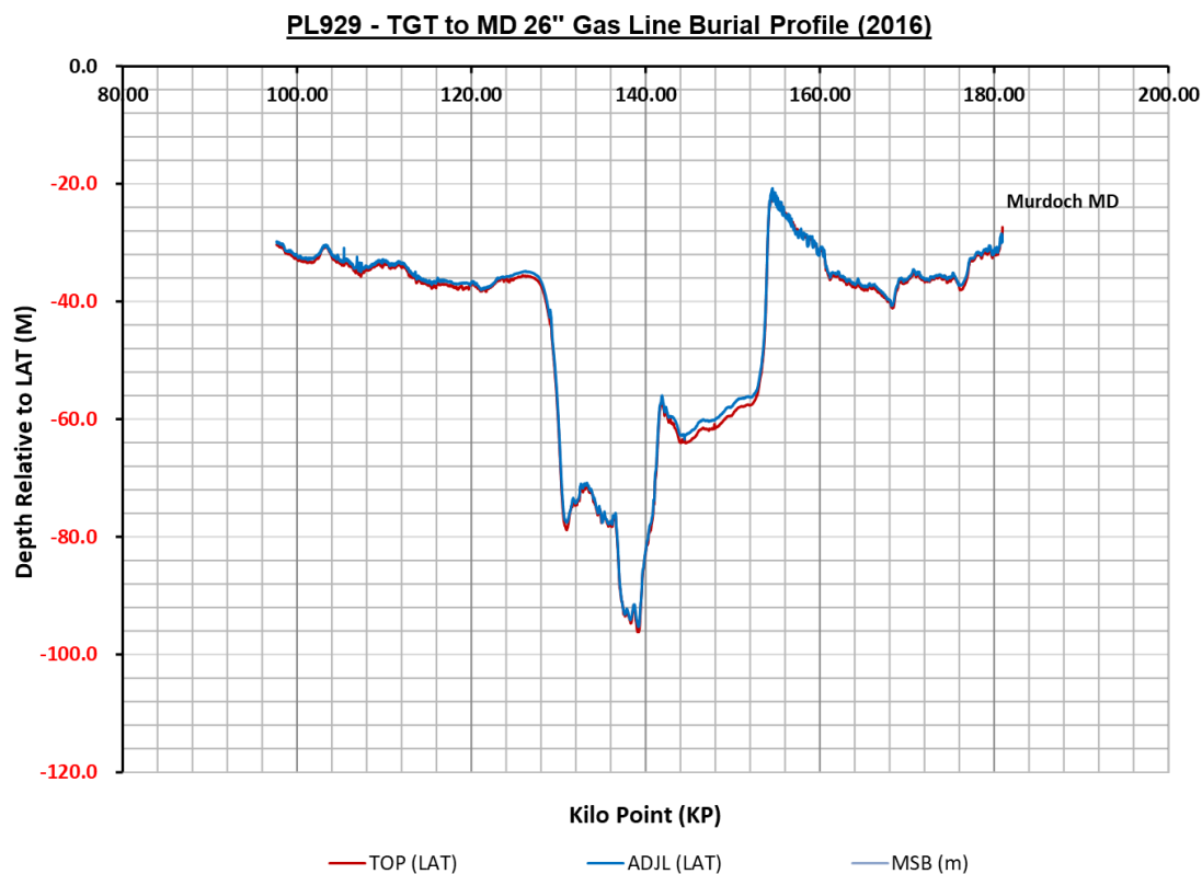
Figure A1.1.3: PL929 seabed & burial profile ~KP97 to ~KP181 (2016)
