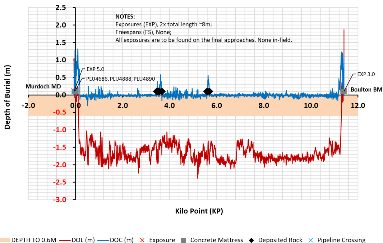
Figure 3.4.2: PL1436 & PL1437 depth of cover profile ~KP-0.06 to ~KP11.41 (2015)
