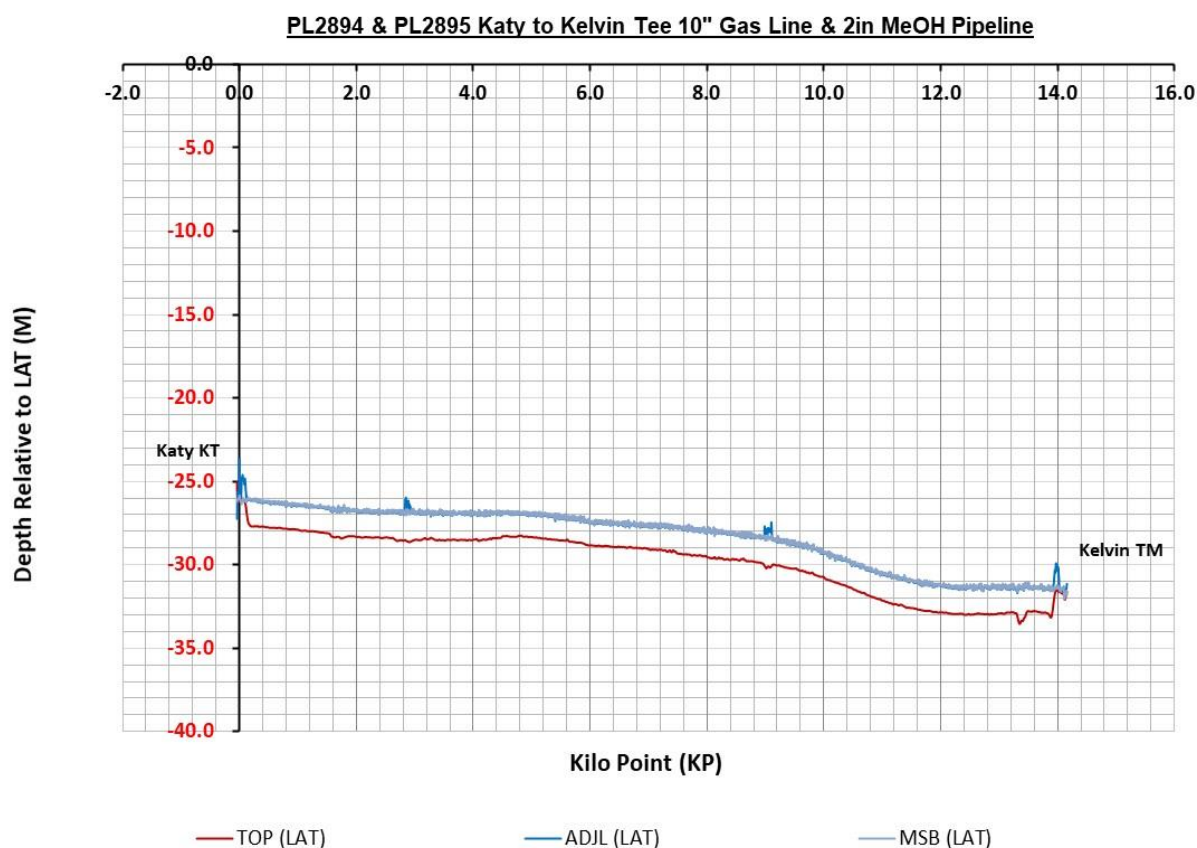
Figure 3.10.1: PL2894 & PL2895 seabed & burial profile ~KP-0.04 to ~KP14.16 (2013)
