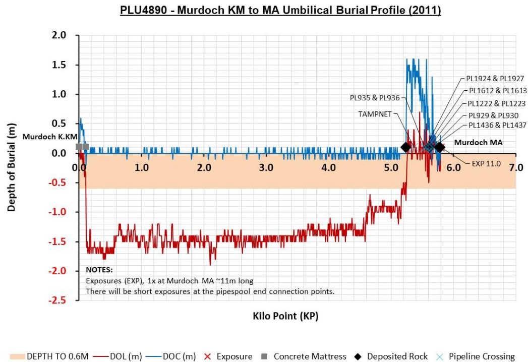
Figure 3.13.2: PLU4890 depth of cover profile ~KP-0.00 to ~KP5.80 (2011)
