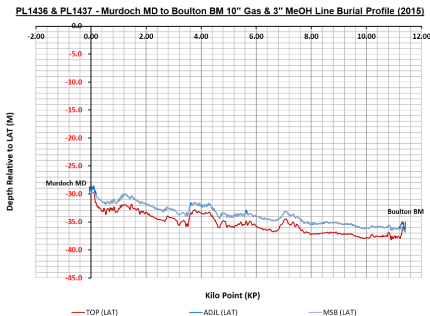
Figure 3.4.1: PL1436 & PL1437 seabed & burial profile ~KP-0.06 to ~KP11.41 (2015)
