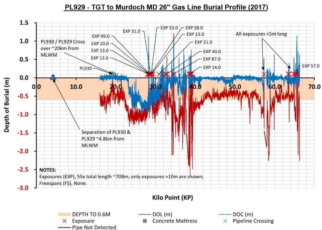
Figure A1.1.2: PL929 depth of cover profile ~KP16 to ~KP66 (2017) 29
