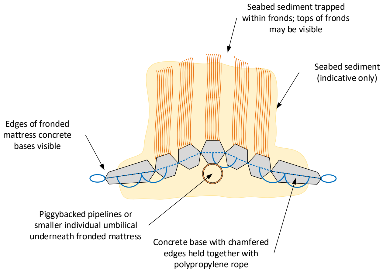
Figure 4.1.2: Fronded mattress with concrete base, edges exposed
