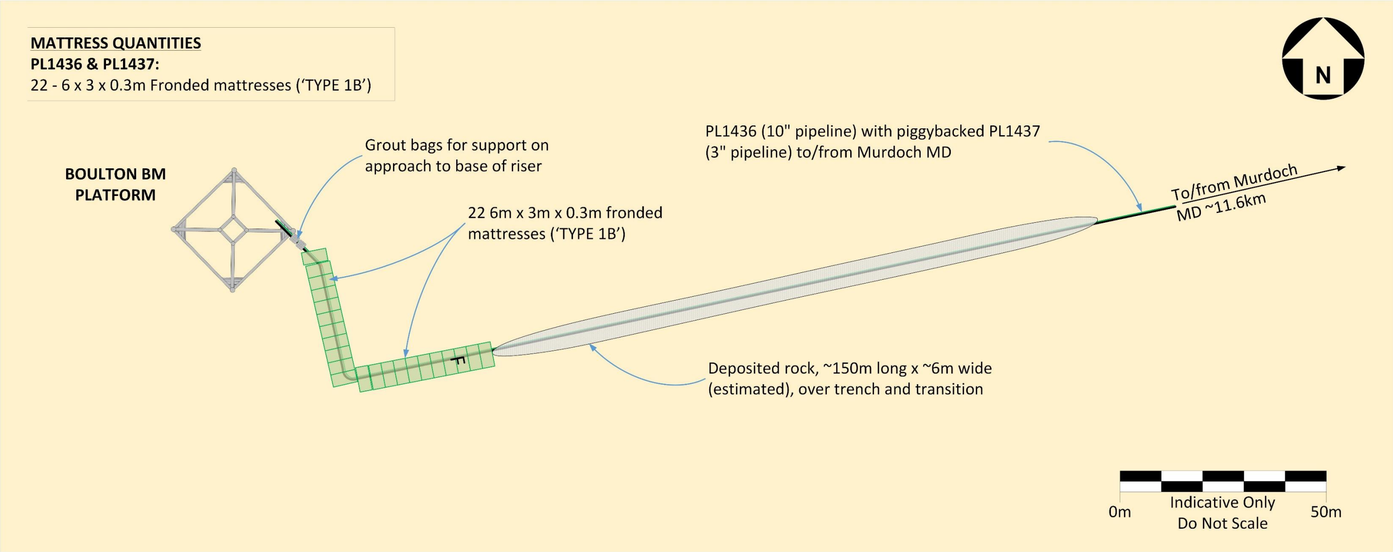
Figure A2.4.1: Schematic of pipelines near Boulton BM
