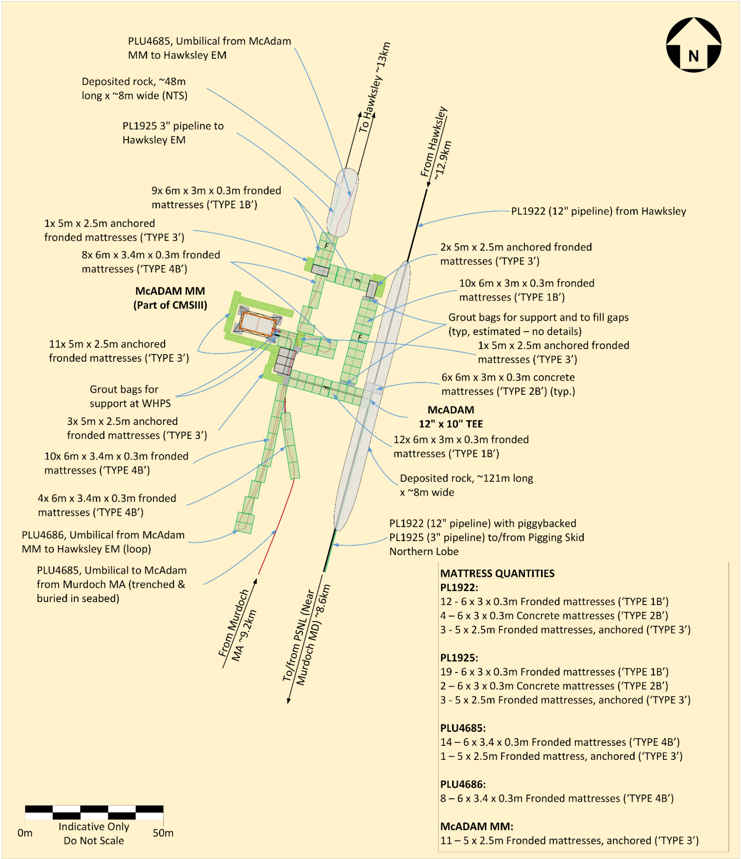
Figure A2.7.1: Schematic of pipelines near McAdam MM
