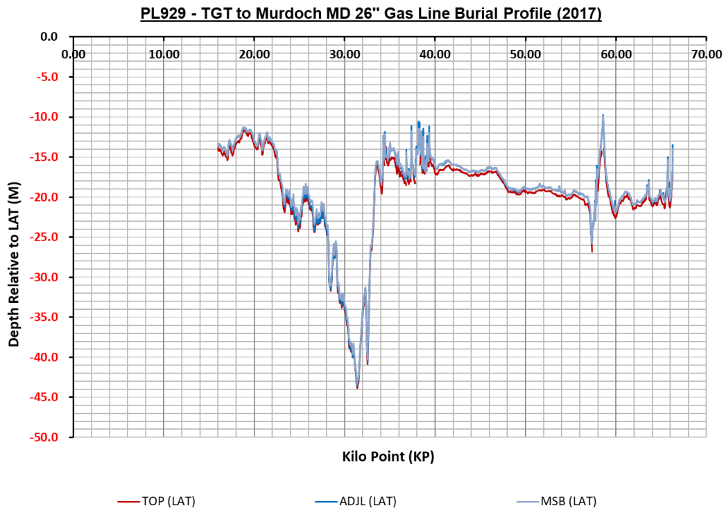
Figure A1.1.1: PL929 seabed & burial profile ~KP16 to ~KP66 (2017)
