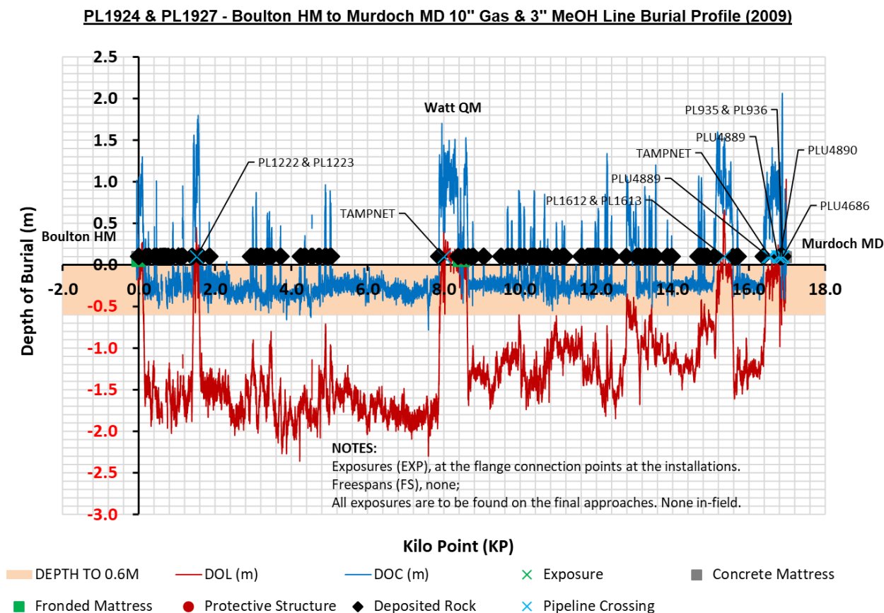
Figure 3.7.2: PL1924 & PL1927 depth of cover profile ~KP-0.05 to ~KP16.98 (2009)
