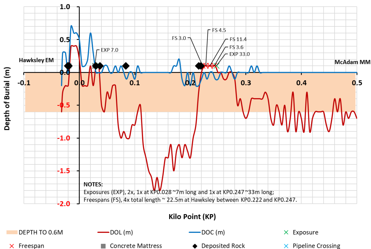
Figure 3.11.6: PLU4685 depth of cover profile ~KP-0.04 to ~KP0.50 (2011) 15
