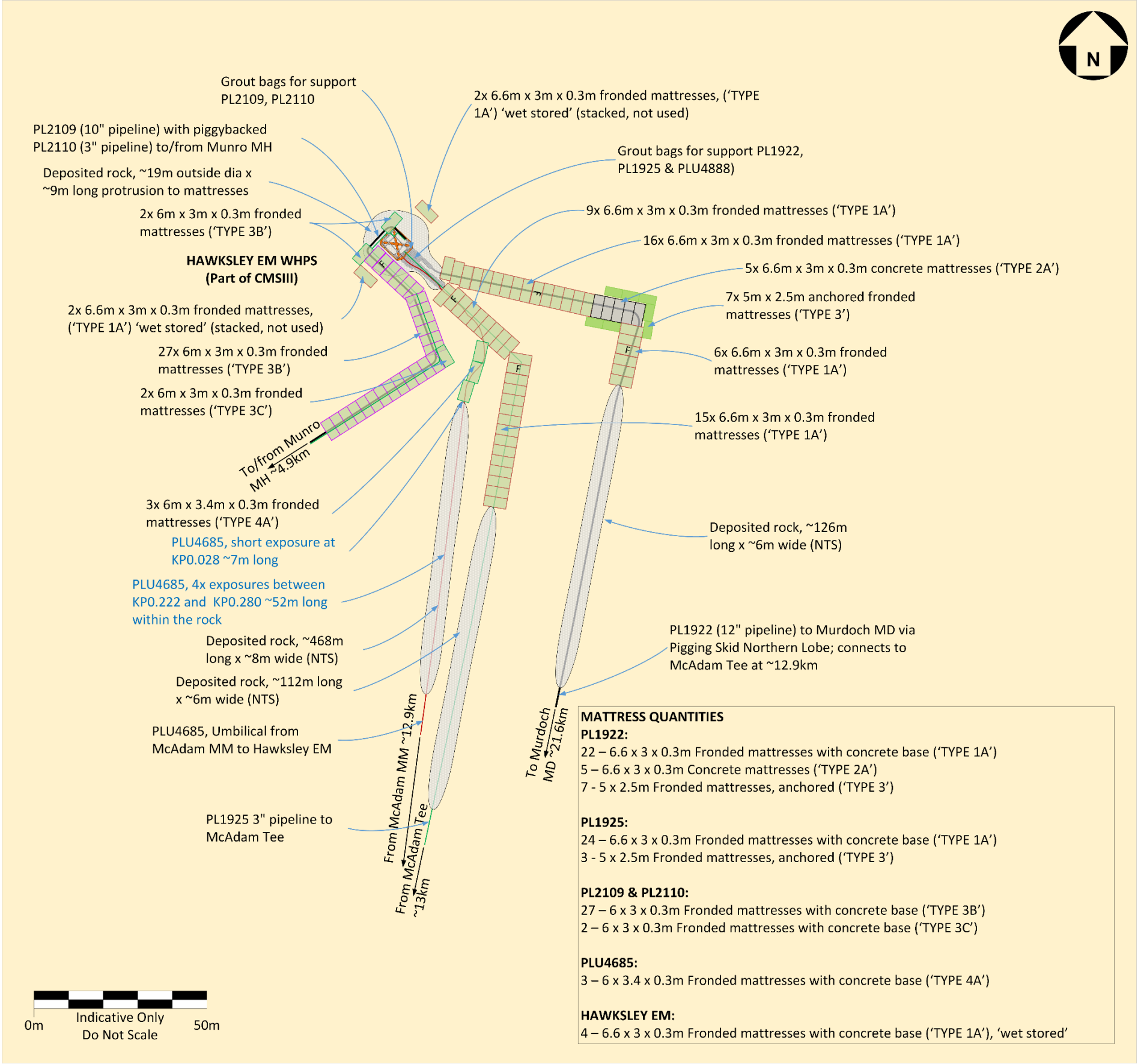
Figure A2.6.1: Schematic of pipelines near Hawksley EM
