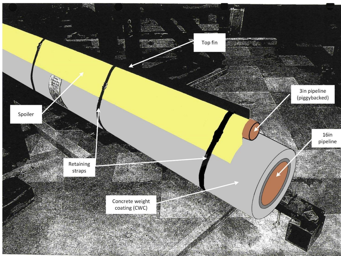
Figure 3.8.1: PL2109 & PL2110 pipeline spoilers
