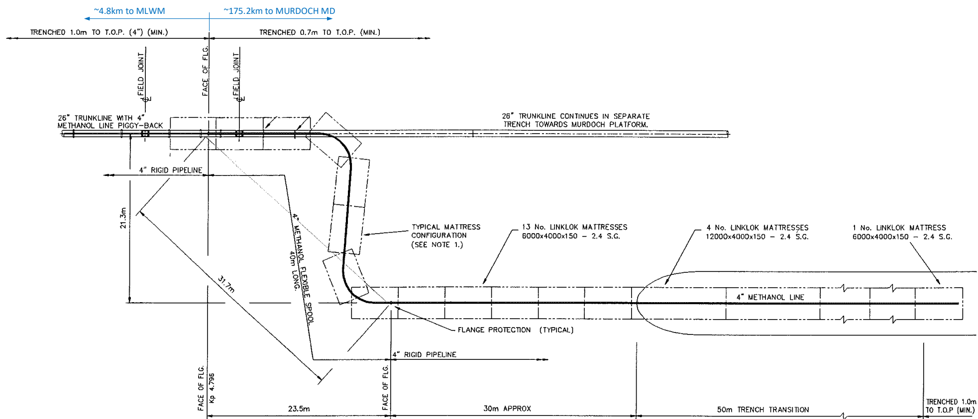
Figure 3.2.4: Separation of PL930 & PL929 ~4.8km from MLWM (NTS)
