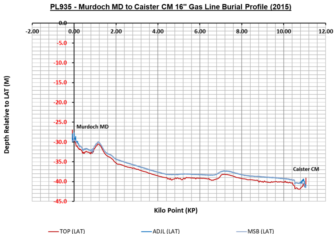
Figure 3.3.1: PL935 seabed & burial profile ~KP-0.1 to ~KP11.1
