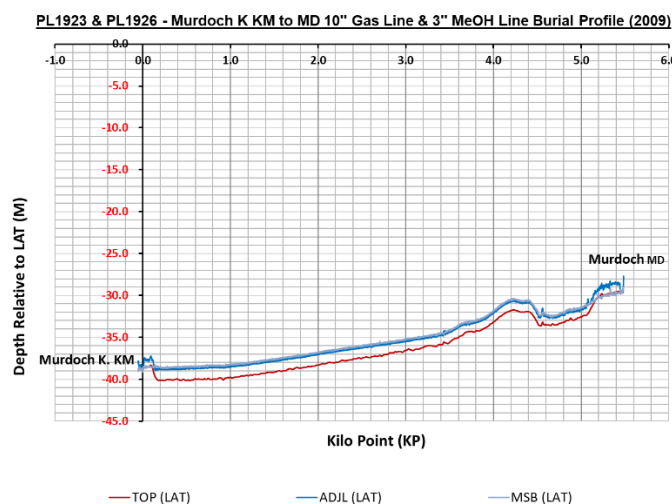
Figure 3.6.1: PL 1923 & PL 1926 seabed & burial profile ~KP-0.05 to ~KP5.49 (2009)
