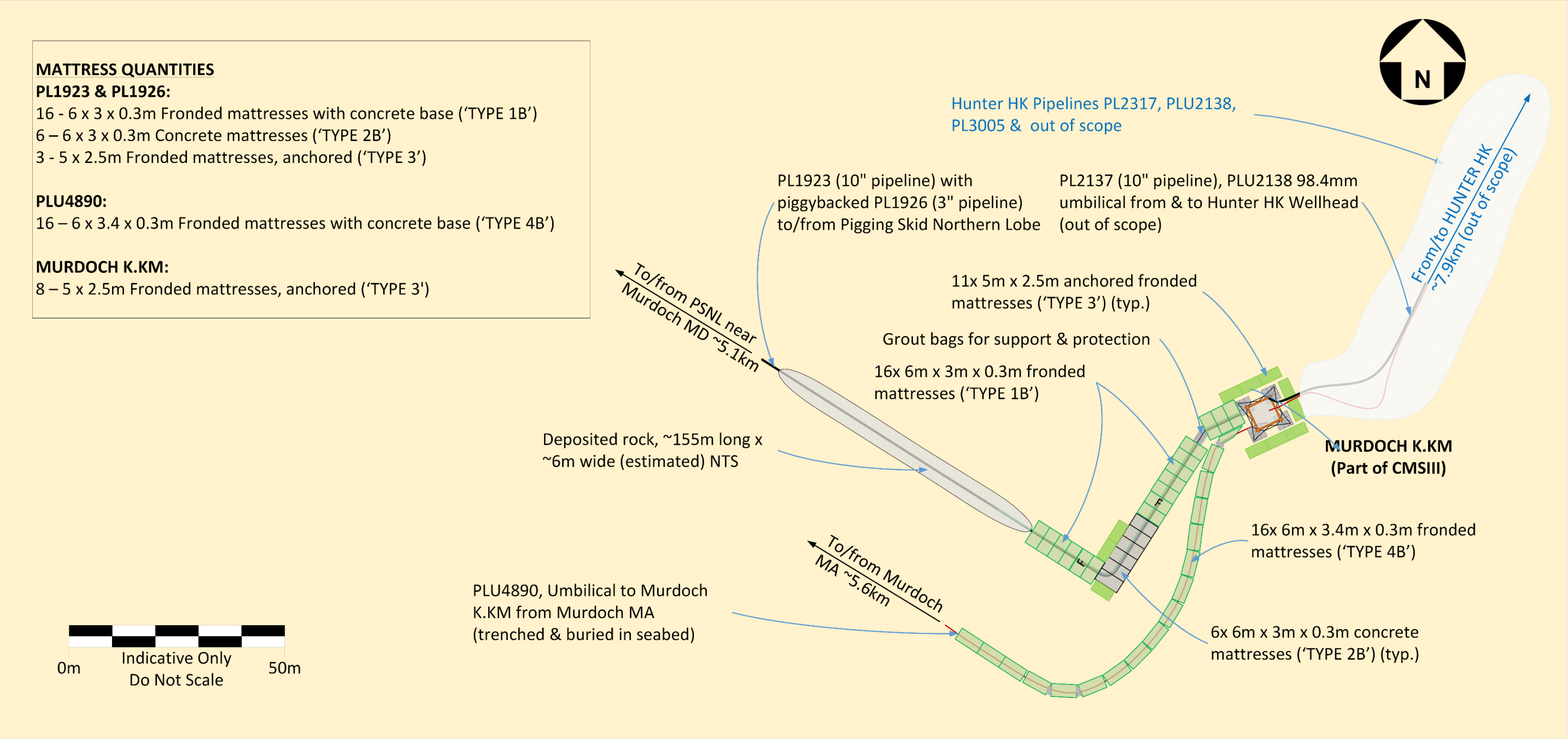
Figure A2.9.1: Schematic of pipelines near Murdoch K.KM
