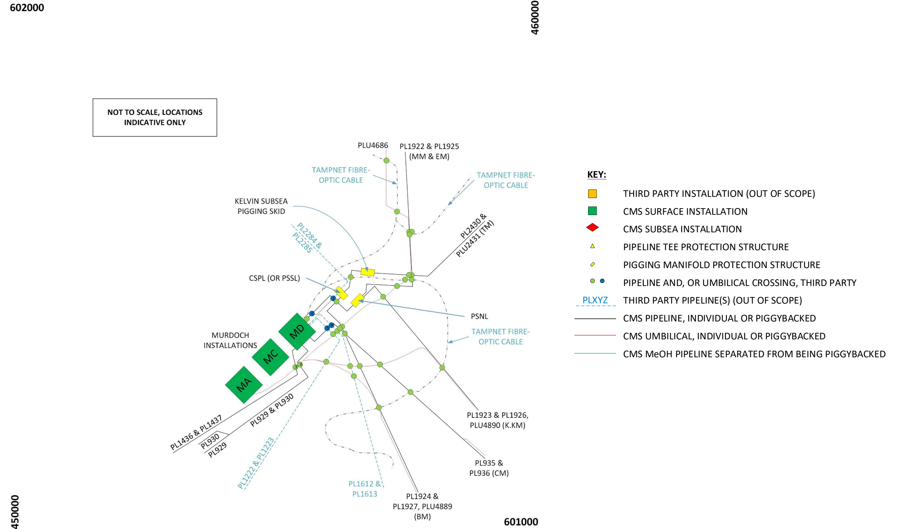
Figure A3.2.1: Schematic of Pipeline Crossings inside Murdoch 500m Zone
