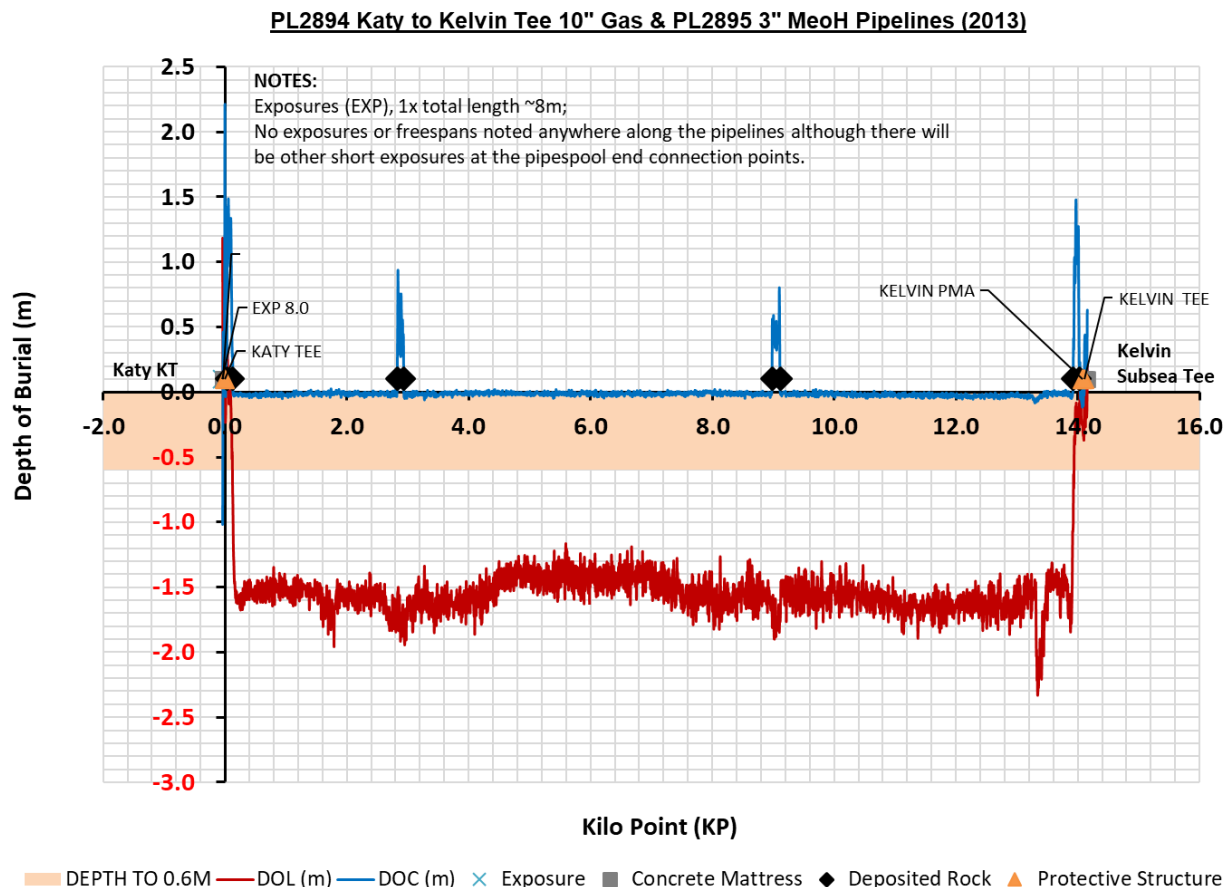
Figure 3.10.2: PL2894 & PL2895 depth of cover profile ~KP-0.04 to ~KP14.16 (2013)
