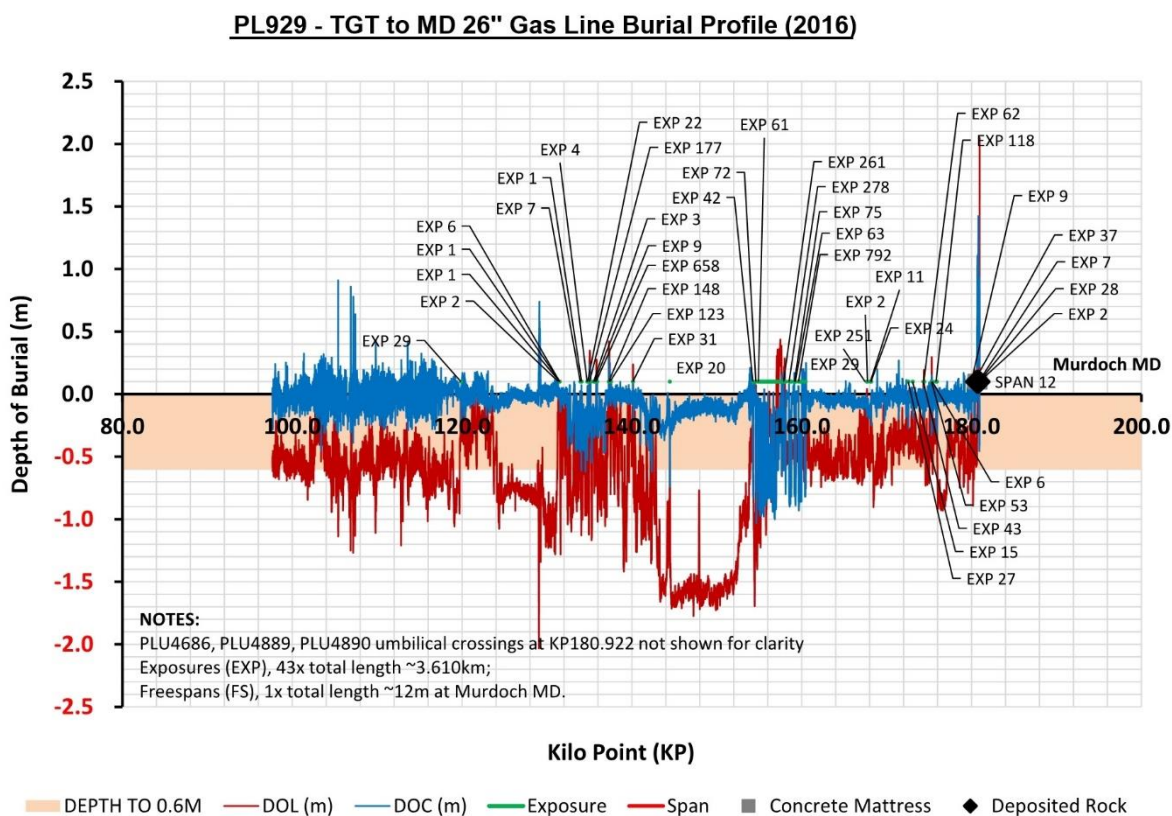
Figure A1.1.4: PL929 depth of cover profile ~KP97 to ~KP181 (2016)
