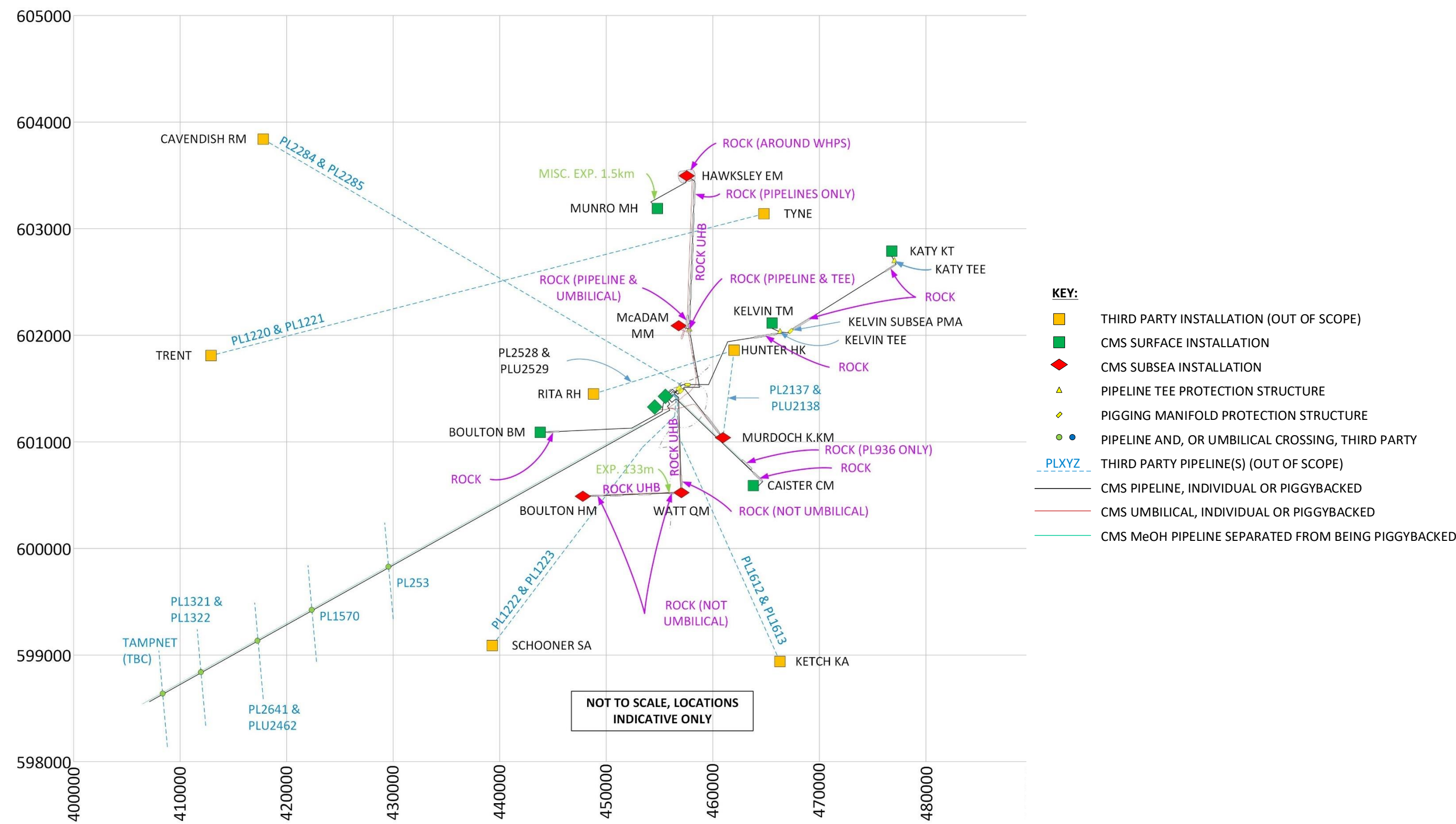
Figure A4.1.1: Schematic of deposited rock outside Murdoch 500m Zone 31
