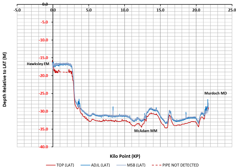
Figure 3.5.1: PL 1922 & PL 1925 seabed & burial profile ~KP-0.085 to ~KP21.75 (2009)
