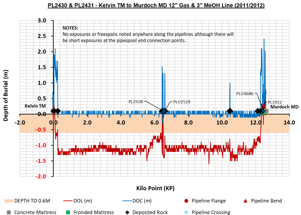
Figure 3.9.2: PL2430 & PLU2431 depth of cover profile ~KP-0.05 to ~KP12.62 (2011/12)
