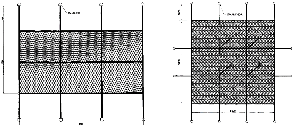
Figure 2.4.4: SPS 5m x 2.5m & 5m x 5m froned mattresses, anchored
