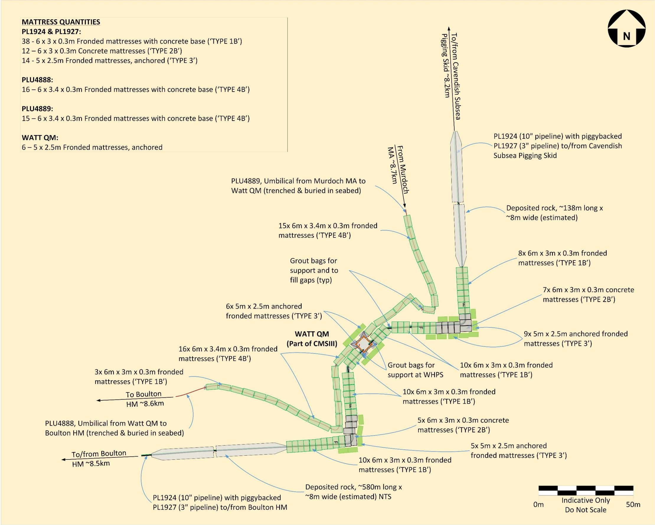
Figure A2.12.1: Schematic of pipelines near Watt QM
