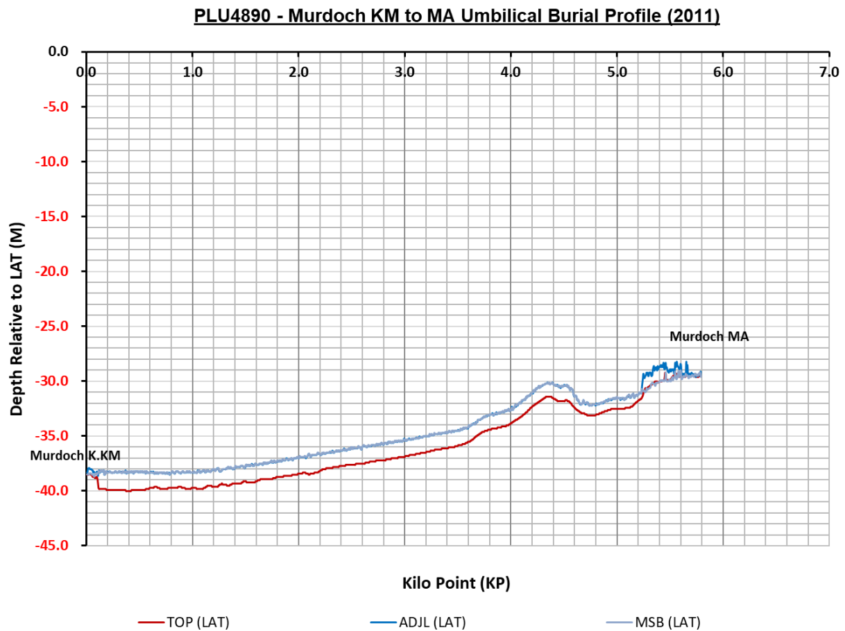
Figure 3.13.1: PLU4890 seabed & burial profile ~KP-0.00 to ~KP5.80 (2011)
