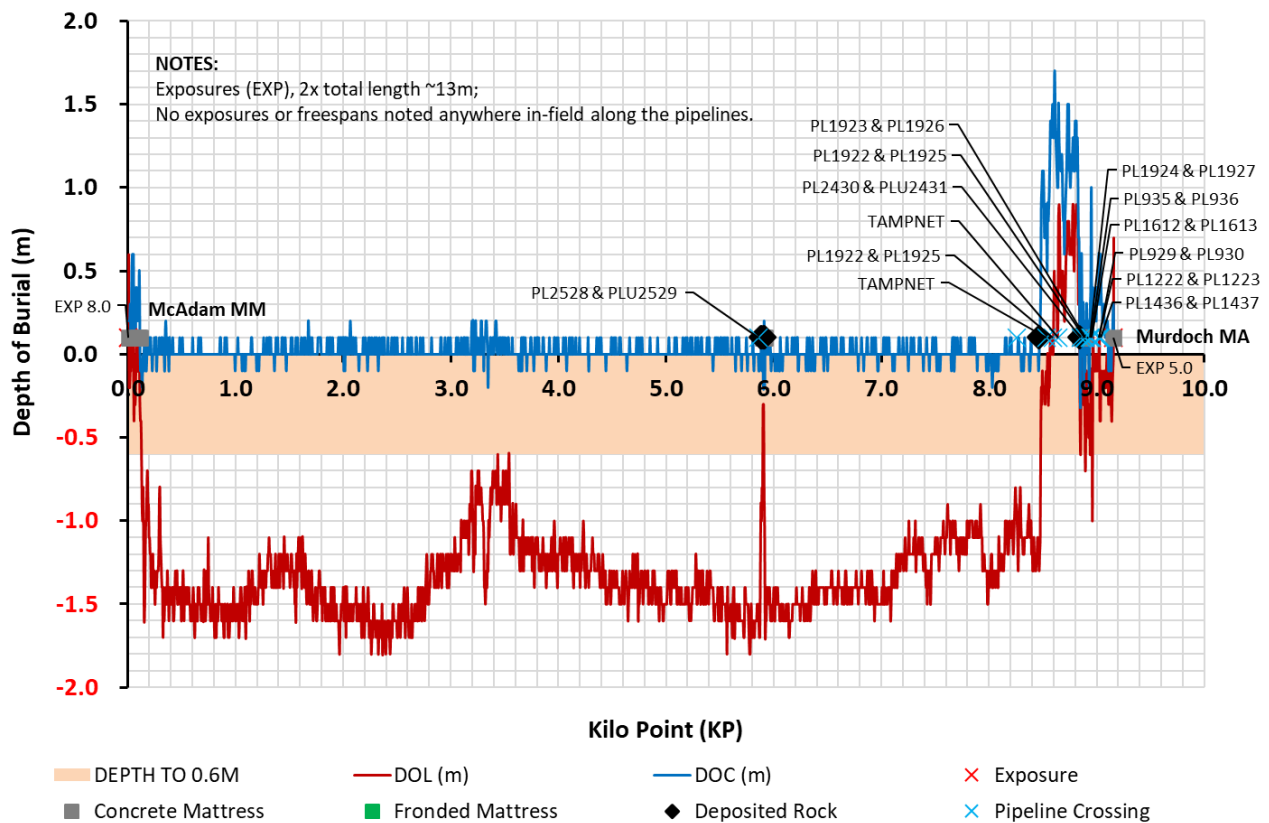
Figure 3.11.2: PLU4686 depth of cover profile ~KP0.0 to ~KP9.16 (2011)
