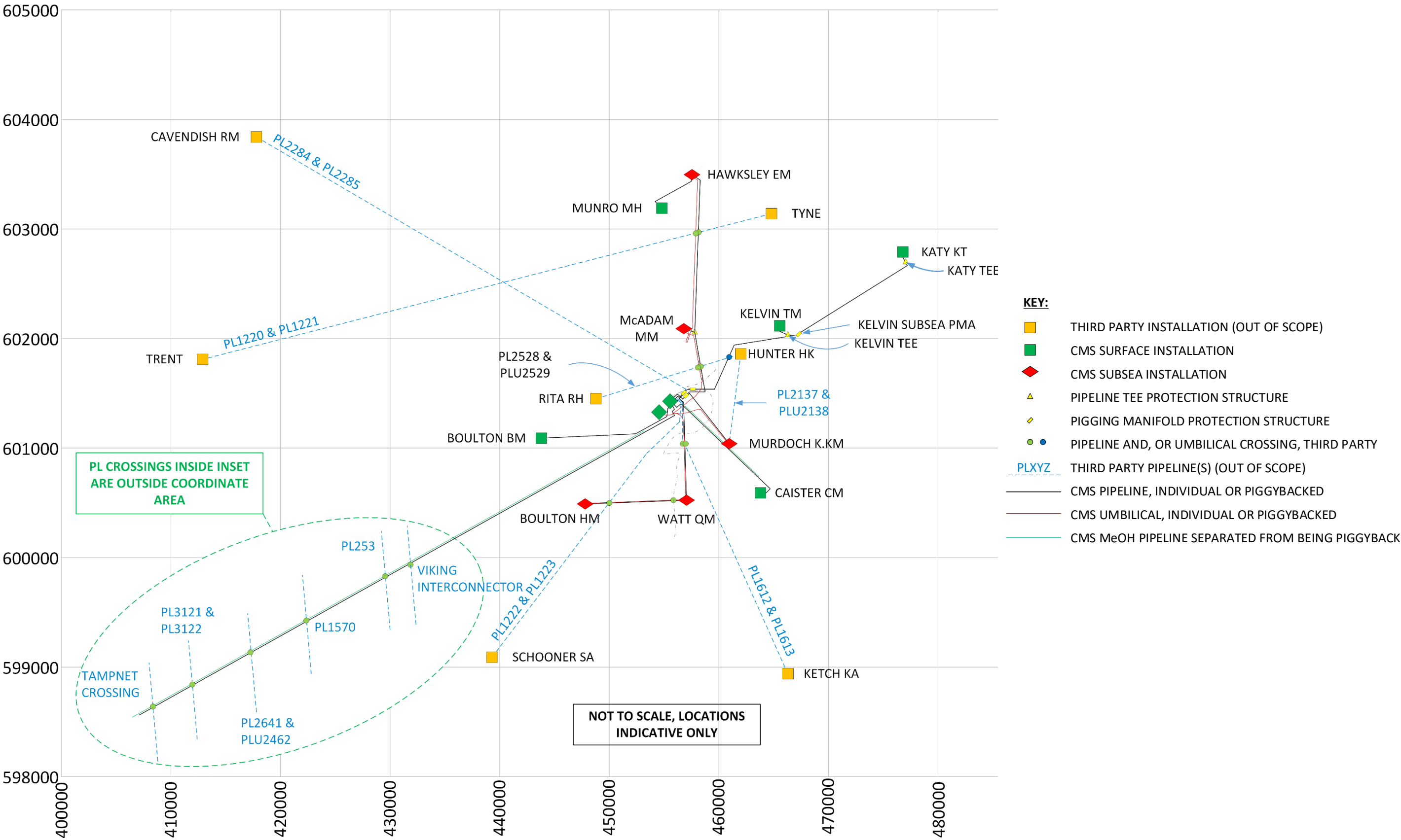
Figure A3.1.1: Schematic of Pipeline Crossings outside Murdoch 500m Zone 30
