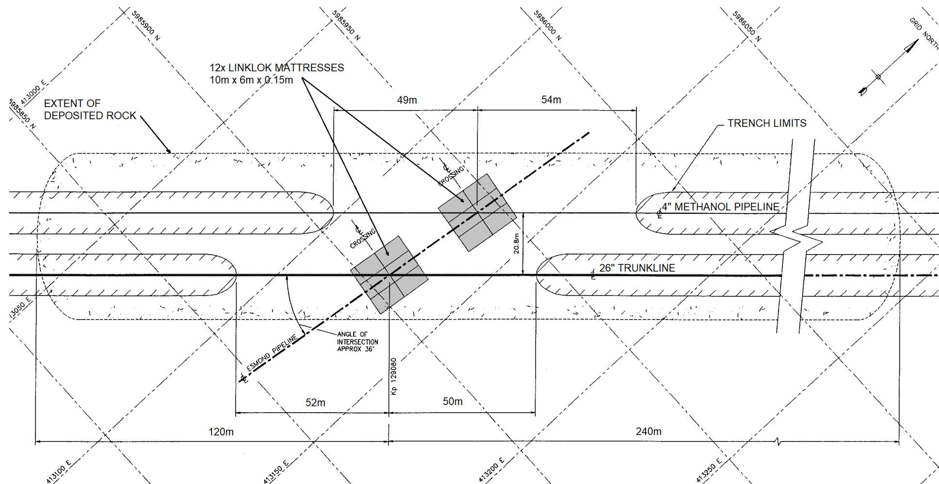
Figure 3.2.2: PL253 Esmond pipeline crossing PL929 & PL930 at ~KP129 (NTS)
