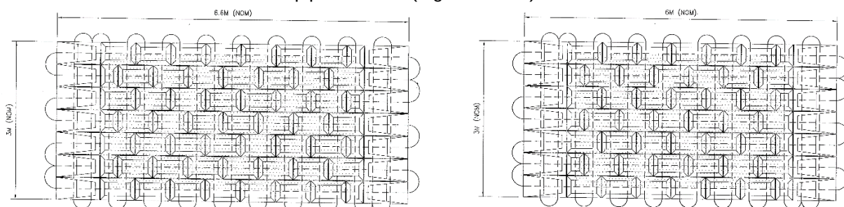
Figure 2.4.5: Froned mattresses Type 6.6m x 3m x 0.3m & 6m x 3m x 0.3m
