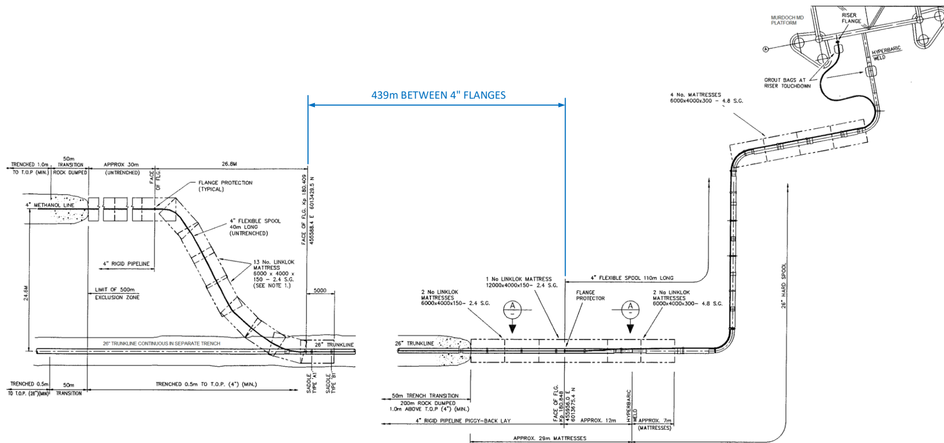
Figure 3.2.1: Separation of PL929 & PL930 at ~500m from Murdoch MD (NTS)
