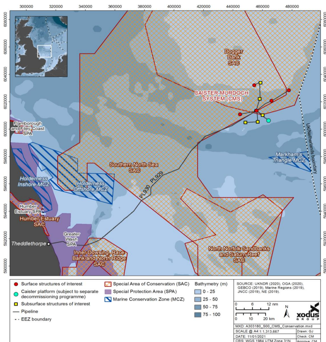
Figure 2.4.1: Oil & Gas Infrastructure with Dogger Bank SAC [1]
