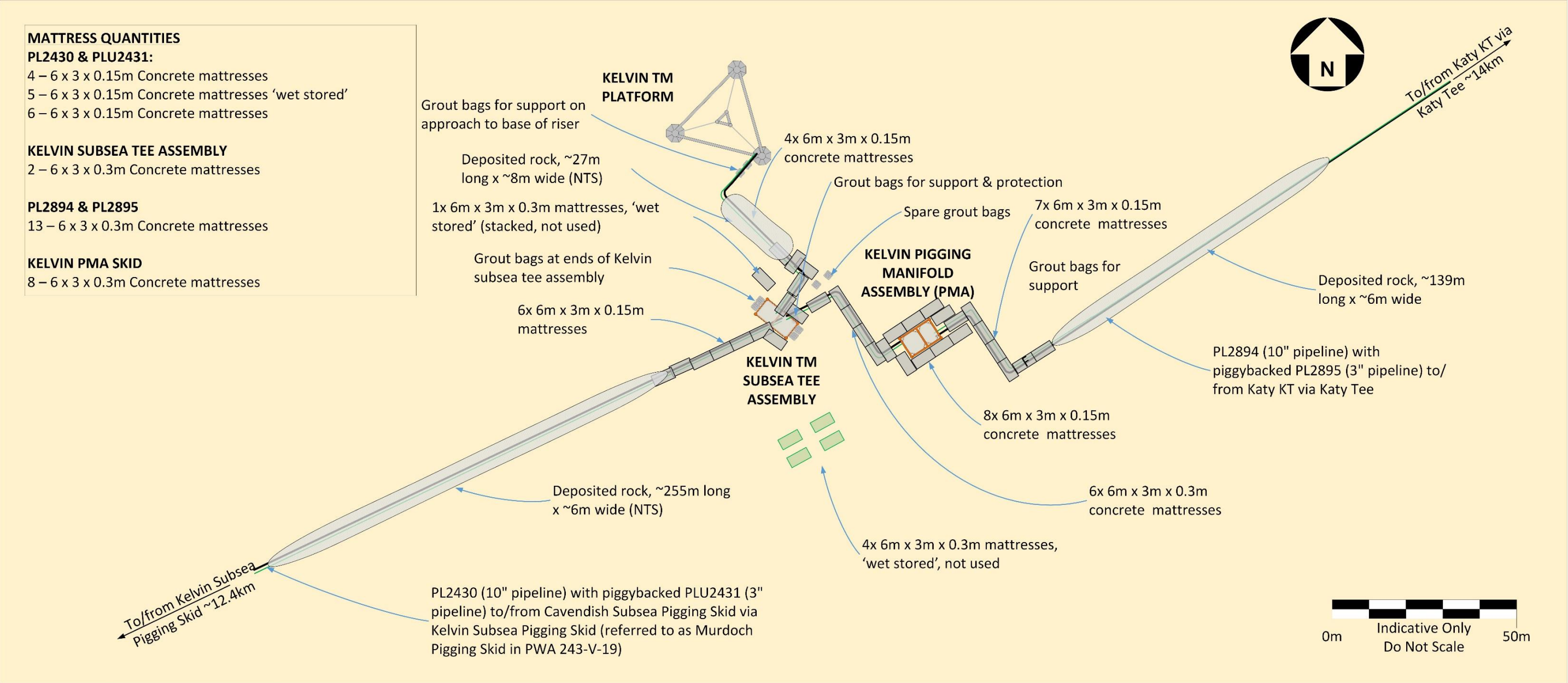
Figure A2.10.1: Schematic of pipelines near Kelvin TM
