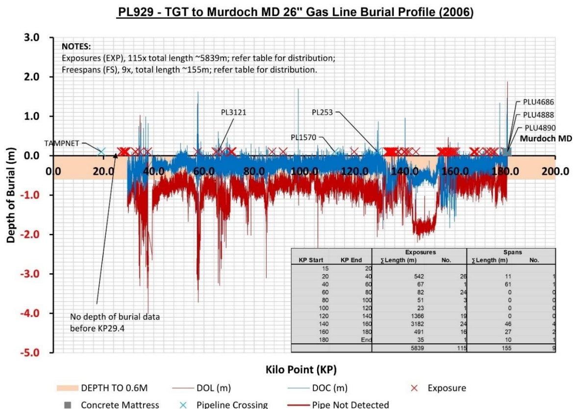
Figure 3.2.6: PL929 depth of cover profile ~KP15 to ~KP181
