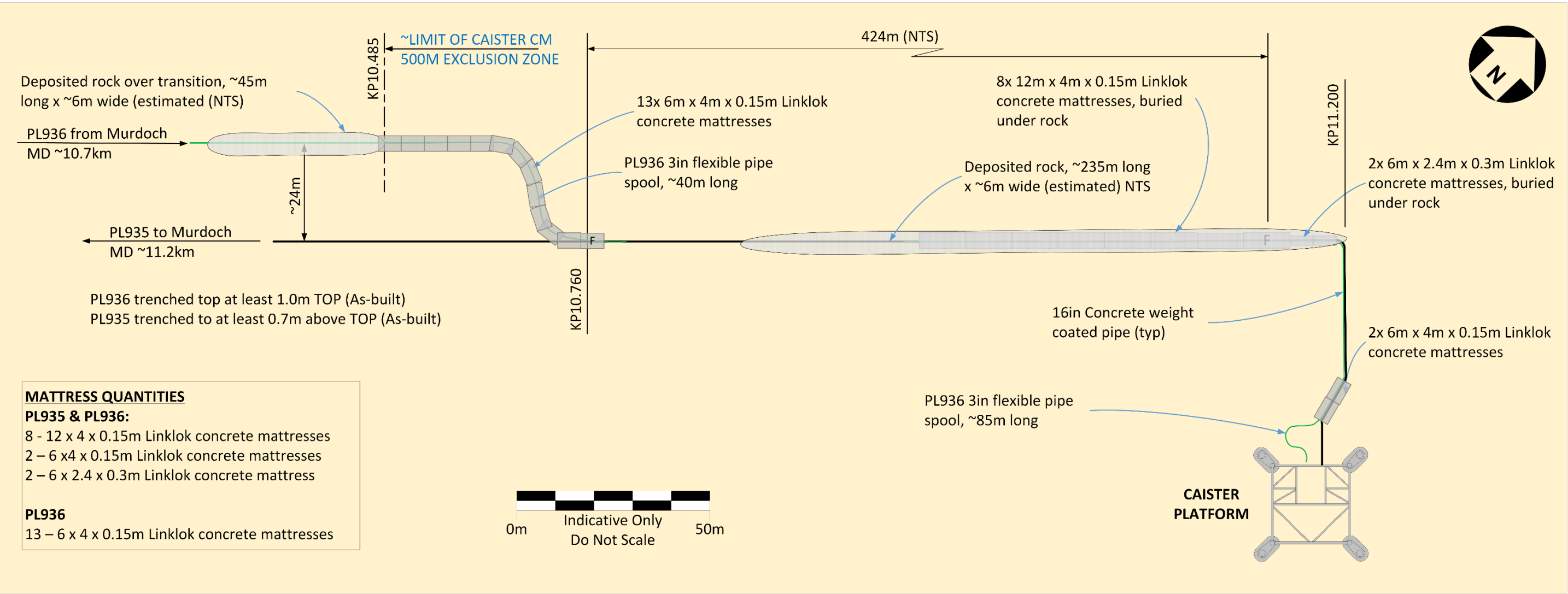
Figure A2.2.1: Schematic of pipelines near Caister CM
