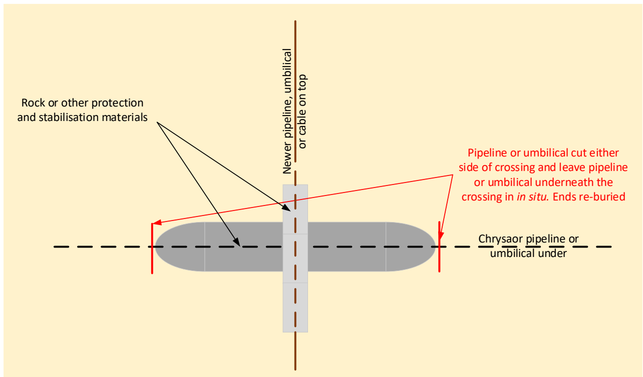
Figure 3.16.1: Pipeline or umbilical being removed from underneath
