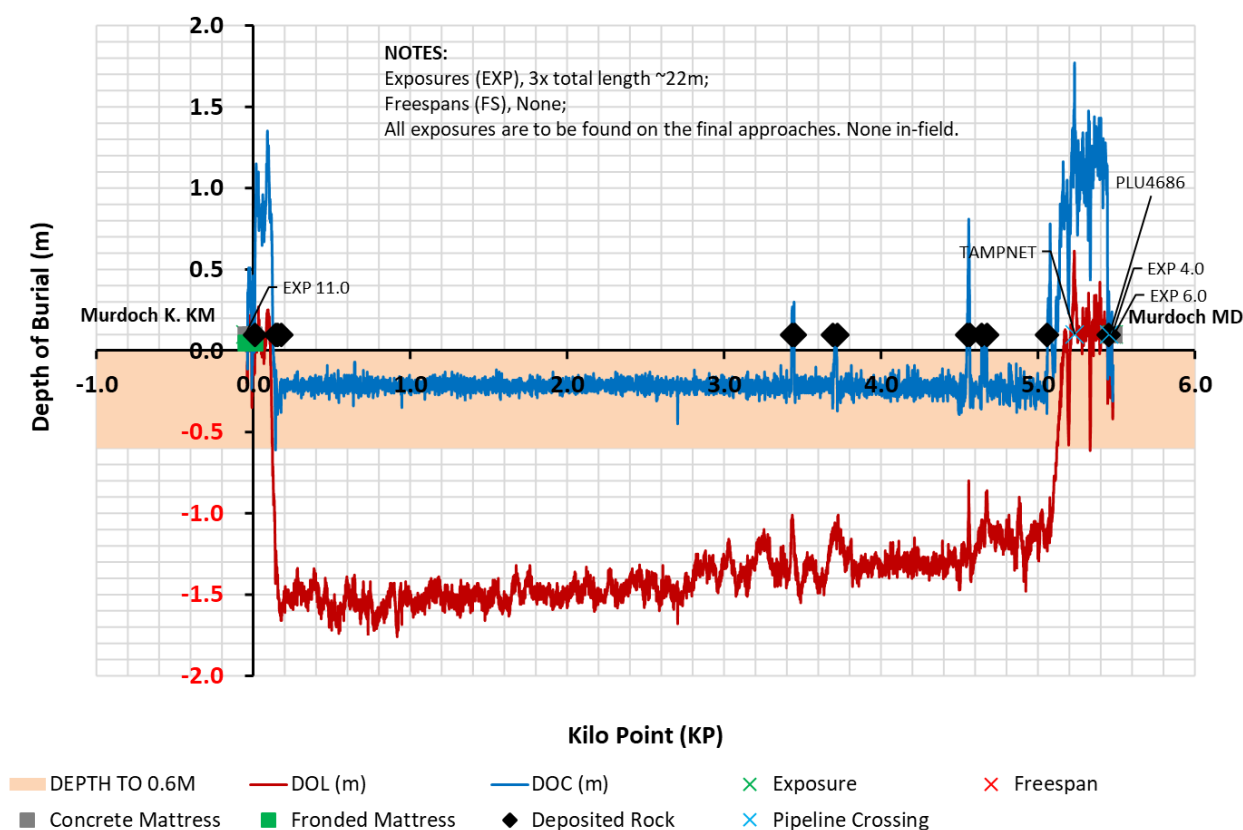
Figure 3.6.2: PL1923 & PL1926 depth of cover profile ~KP-0.05 to ~KP5.49 (2009)
