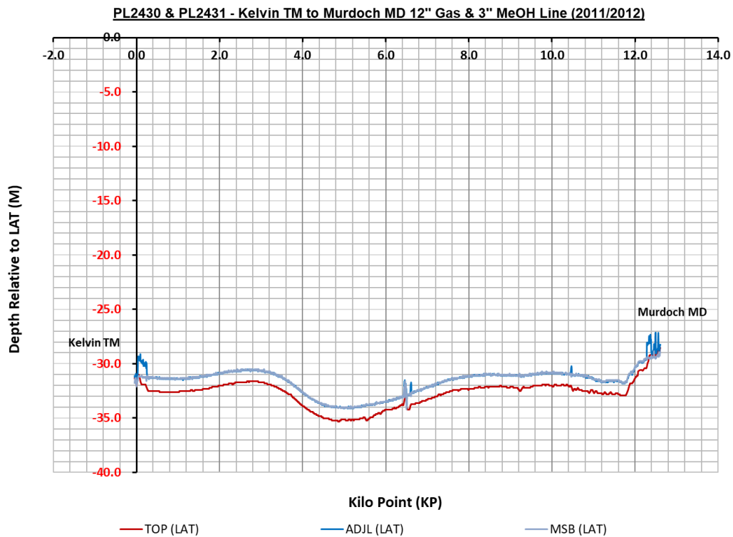
Figure 3.9.1: PL2430 & PLU2431 seabed & burial profile ~KP-0.05 to ~KP12.62 (2011/12)
