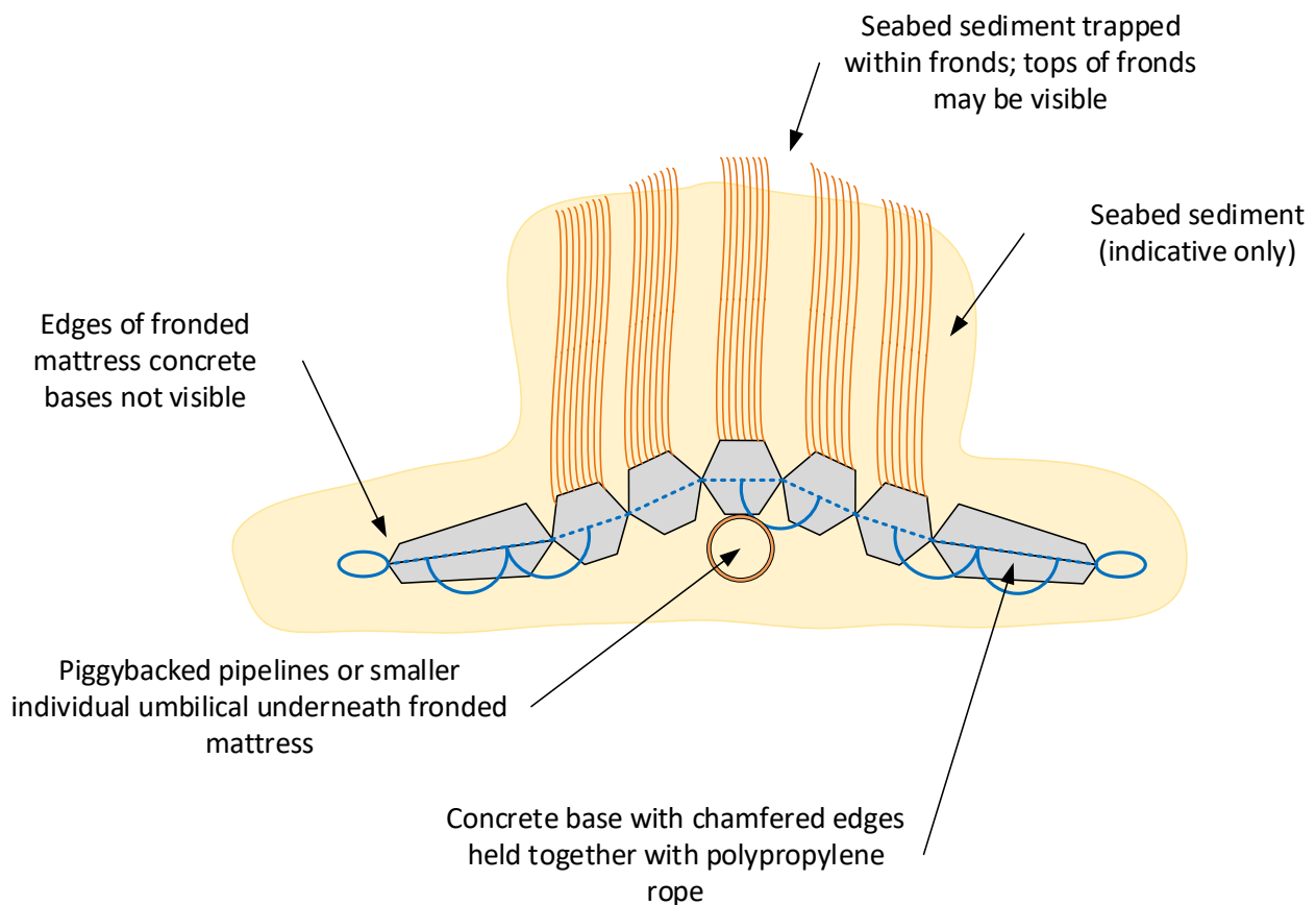
Figure 4.1.1: Fronded mattress with concrete base, edges buried
