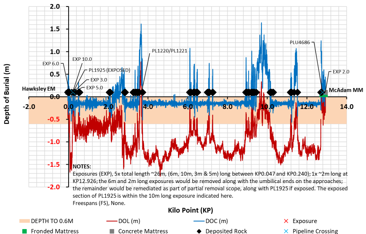
Figure 3.11.3: PLU4685 depth of cover profile ~KP-0.04 to ~KP13 (2007) 14
