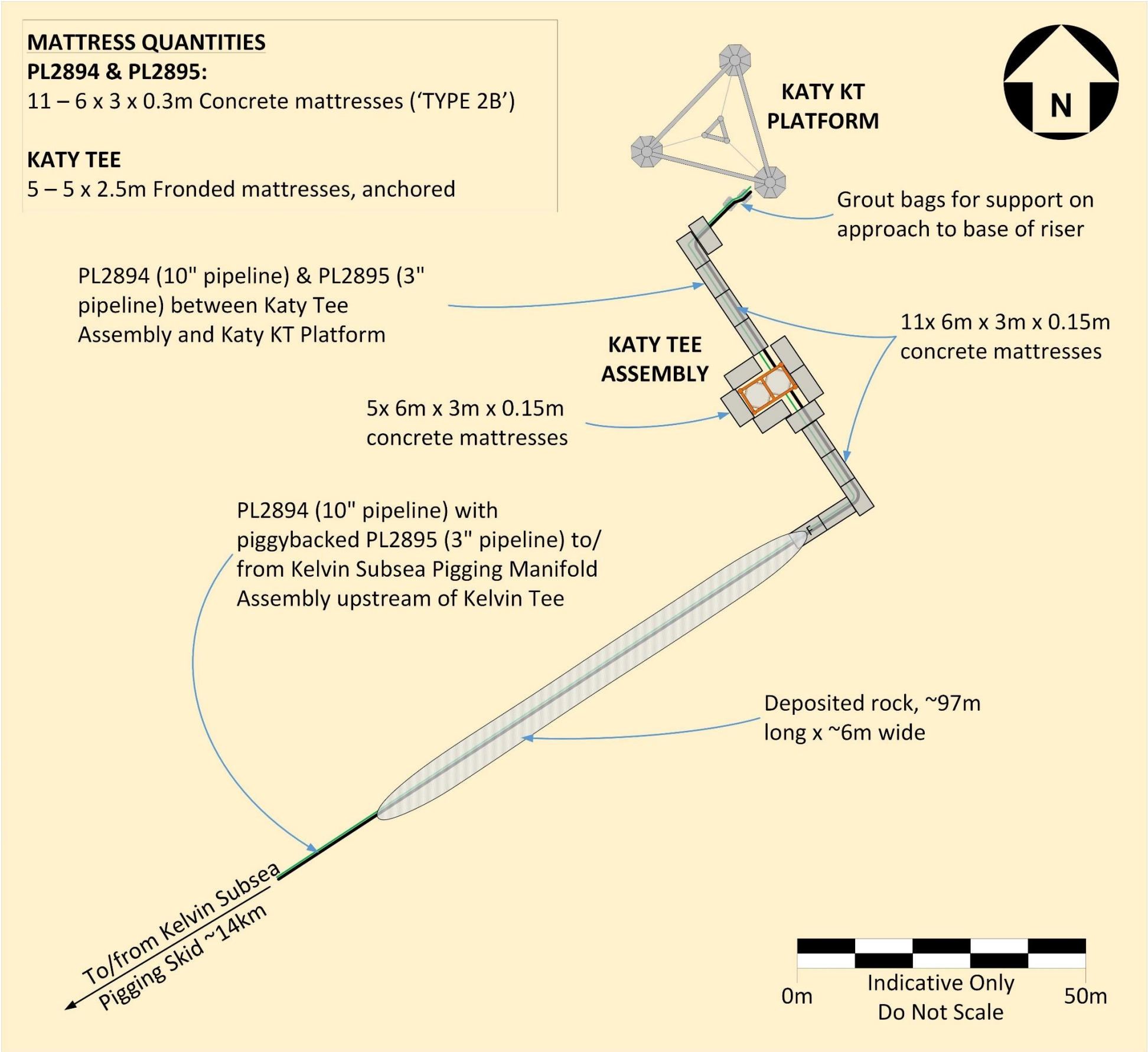
Figure A2.11.1: Schematic of pipelines near Katy KT
