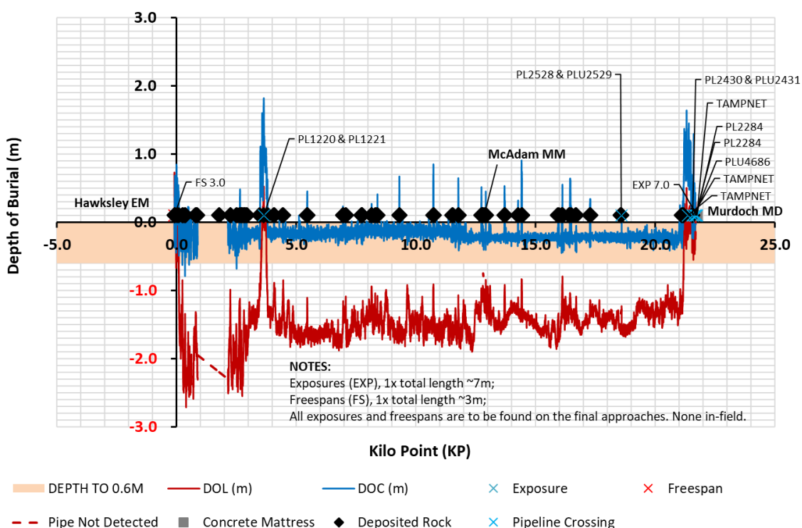
Figure 3.5.2: PL 1922 & PL 1925 depth of cover profile ~KP-0.08 to ~KP21.75 (2009)
