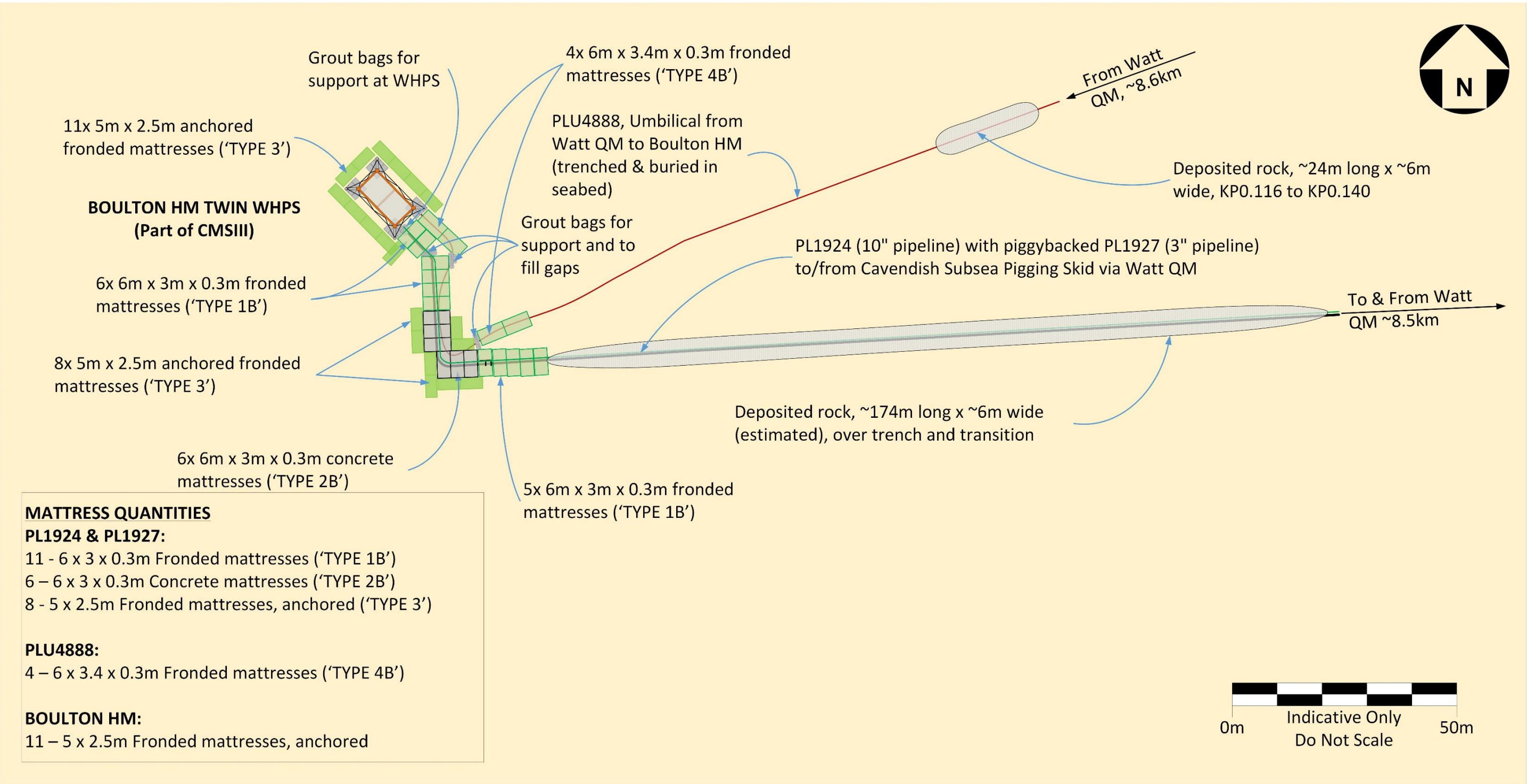
Figure A2.5.1: Schematic of pipelines near Boulton HM
