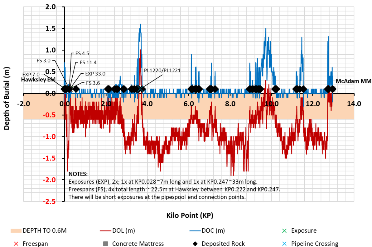
Figure 3.11.5: PLU4685 depth of cover profile ~KP-0.04 to ~KP13 (2011)
