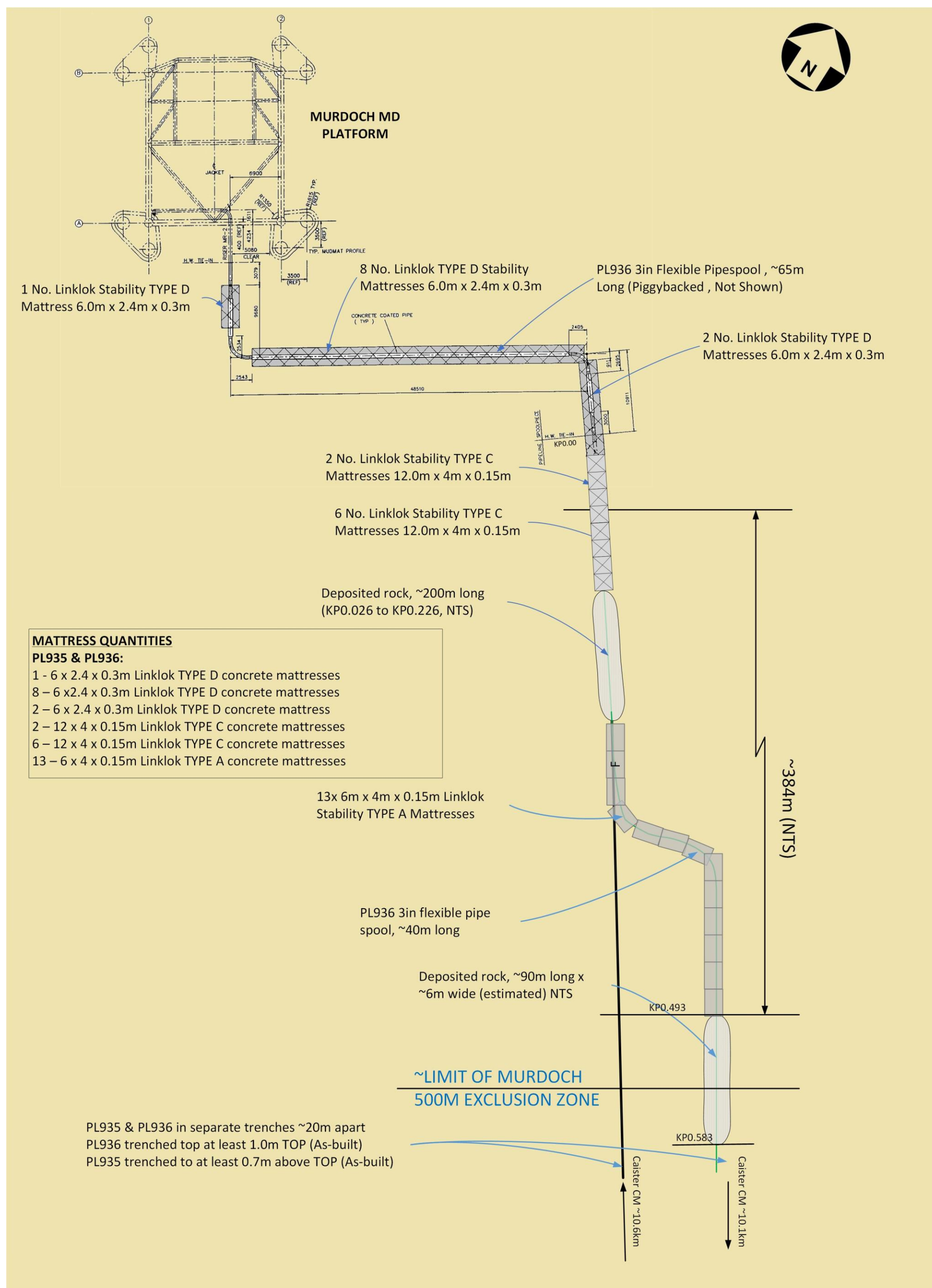
Figure A2.3.1: Schematic of PL935 & PL936 near Murdoch MD
