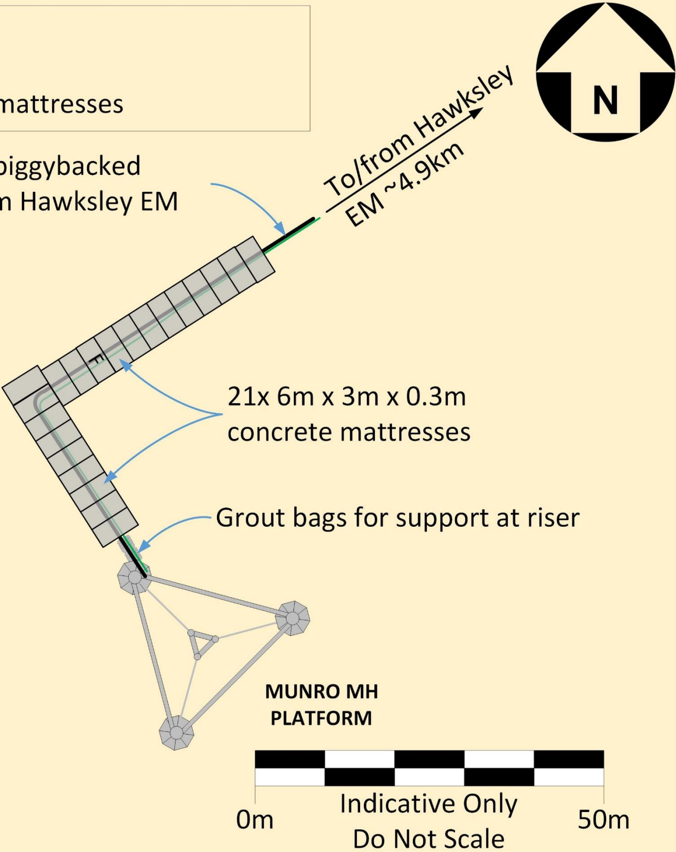
Figure A2.8.1: Schematic of pipelines near Munro MH
