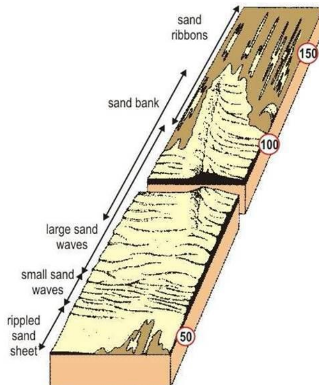
Figure 2.4.2: Sand waves and sand banks [4] 9
