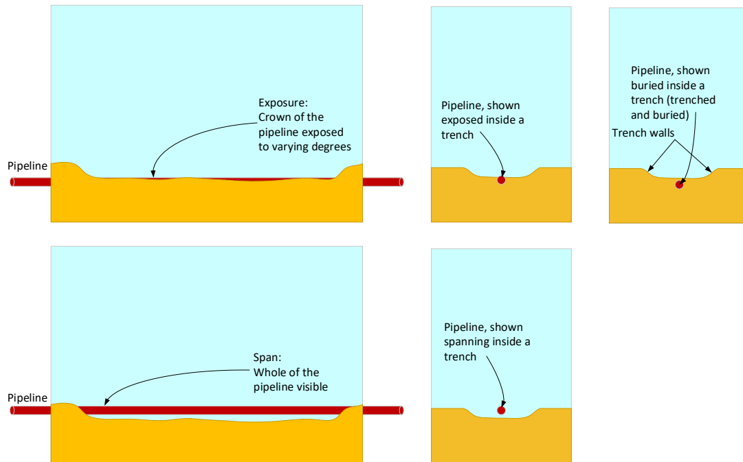
Figure 3.14.1: The difference between pipeline exposures and spans 16
