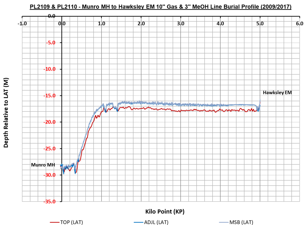
Figure 3.8.2: PL2109 & PL2110 seabed & burial profile ~KP-0.05 to ~KP16.98 (2009/17)
