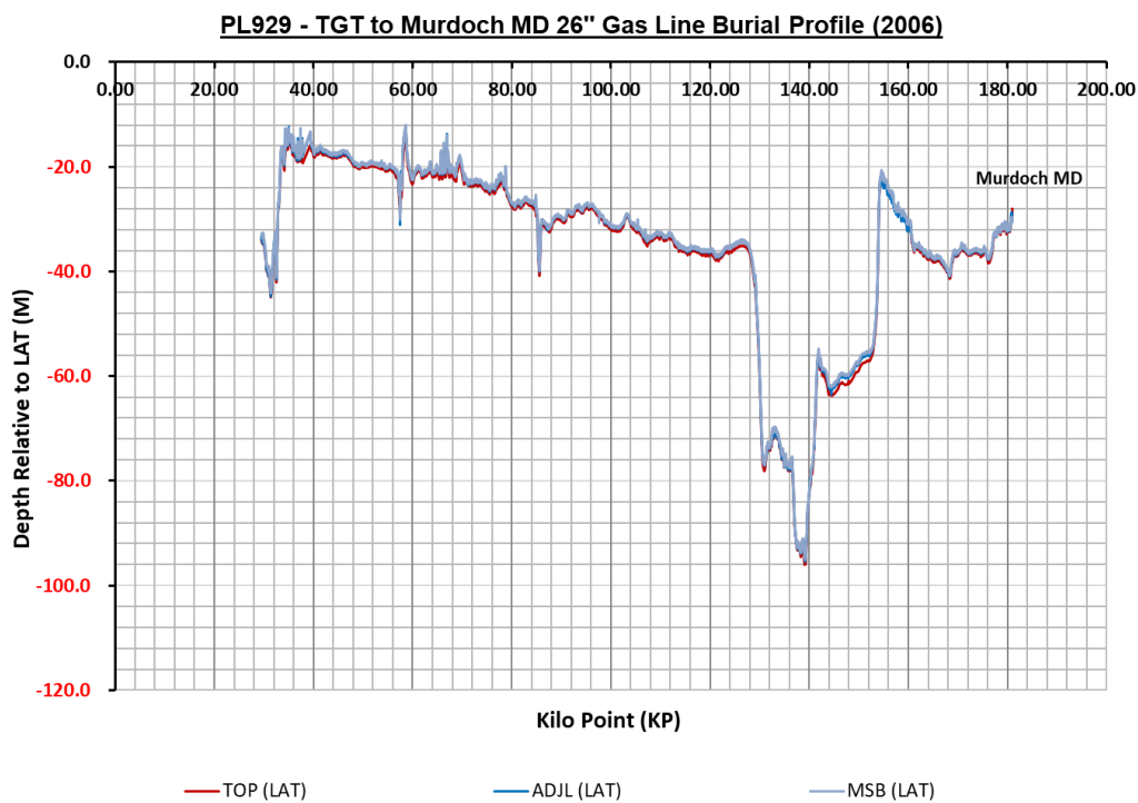
Figure 3.2.5: PL929 seabed & burial profile ~KP15 to ~KP181
