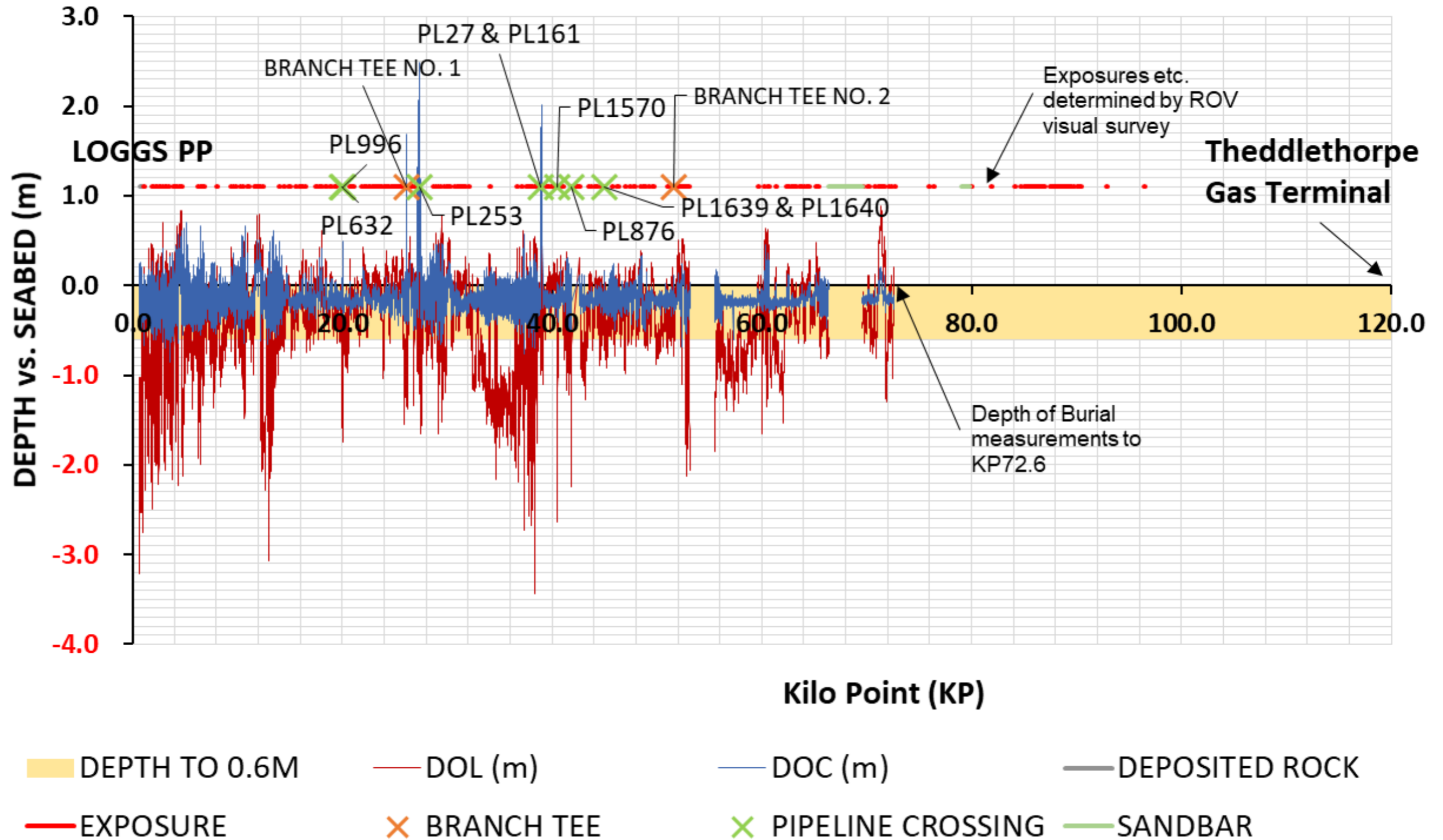
Figure A1.1.2: PL454 Depth of Cover Profile (2010-2018) 11
