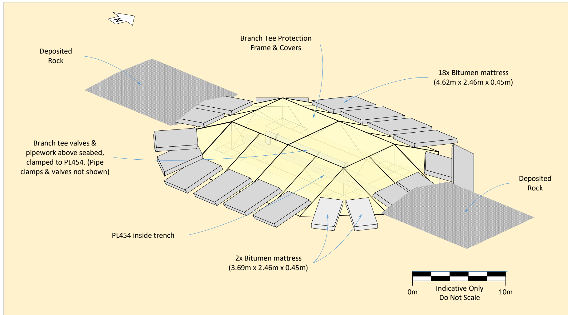
Figure 2.3.2: Schematic Branch Tee No. 1 5
