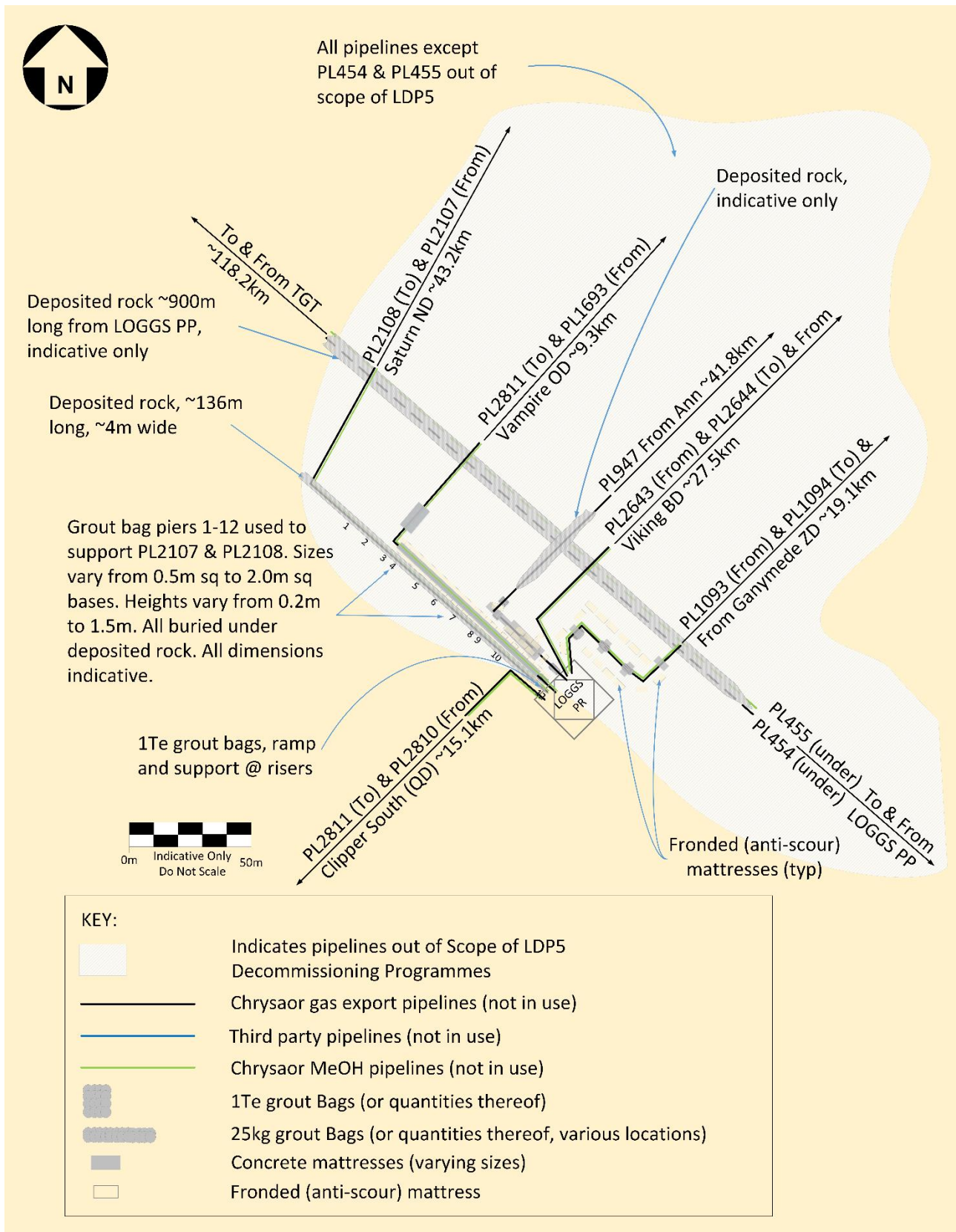
Figure 2.3.6: PL454 & PL455 underneath Third-Party Pipelines at LOGGS PR
