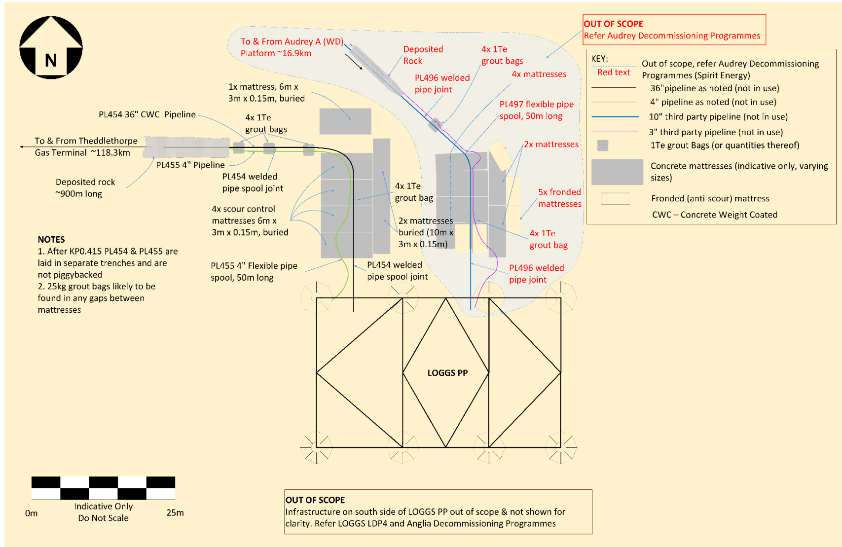
Figure 2.3.7: Approaches & Pipelines LOGGS PP North Side
