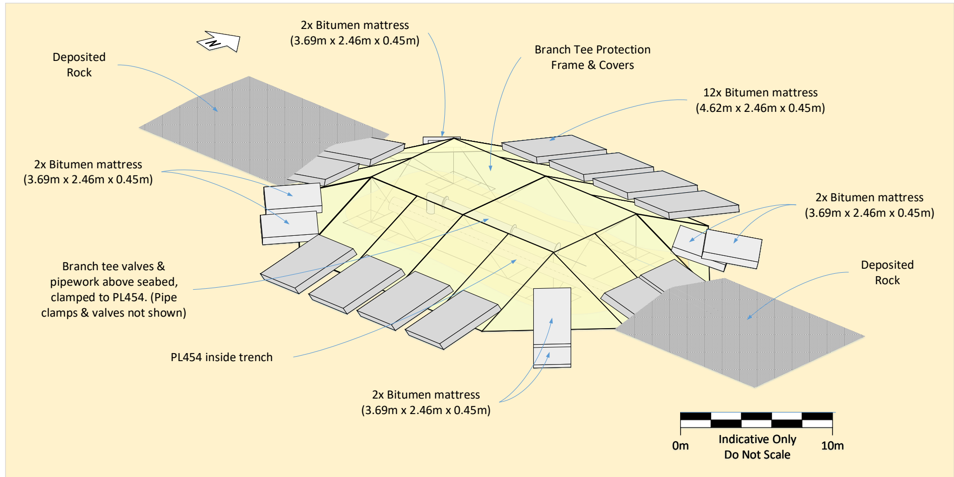
Figure 2.3.3: Schematic Branch Tee No. 2
