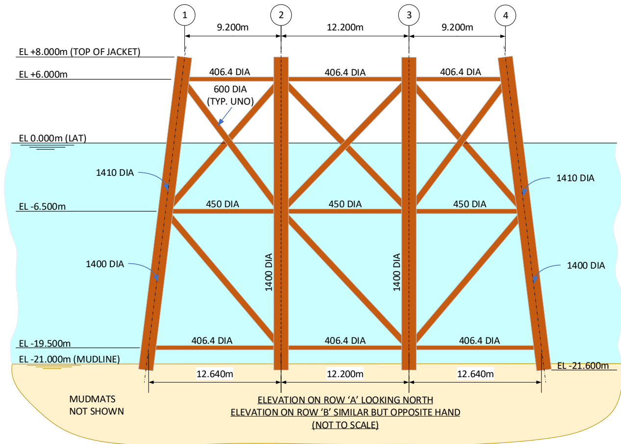
Figure 3.2.5: LOGGS PP Jacket View Looking North
