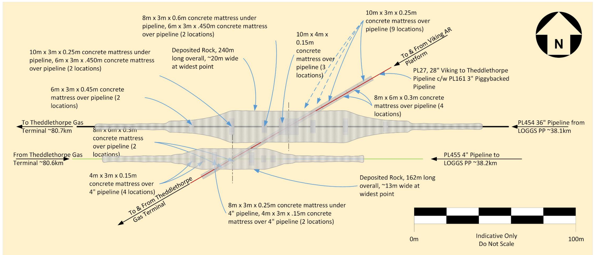
Figure 2.3.5: Pipeline Crossing PL454 & PL455 over PL27 & PL161
