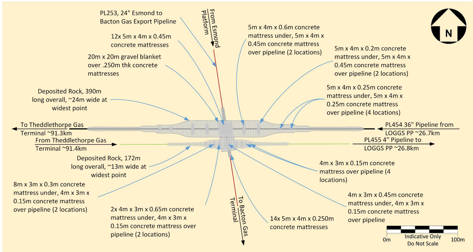
Figure 2.3.4: Pipeline Crossing PL454 & PL455 over PL253
