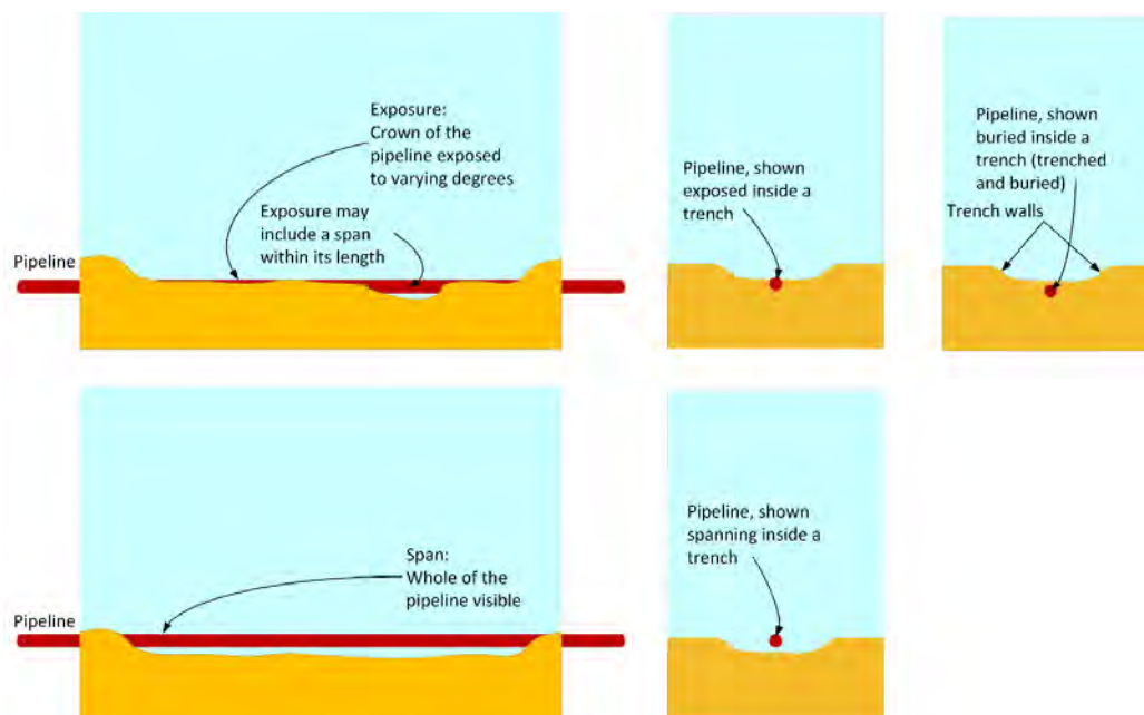
The difference between pipeline burial, exposures, and spans 1
