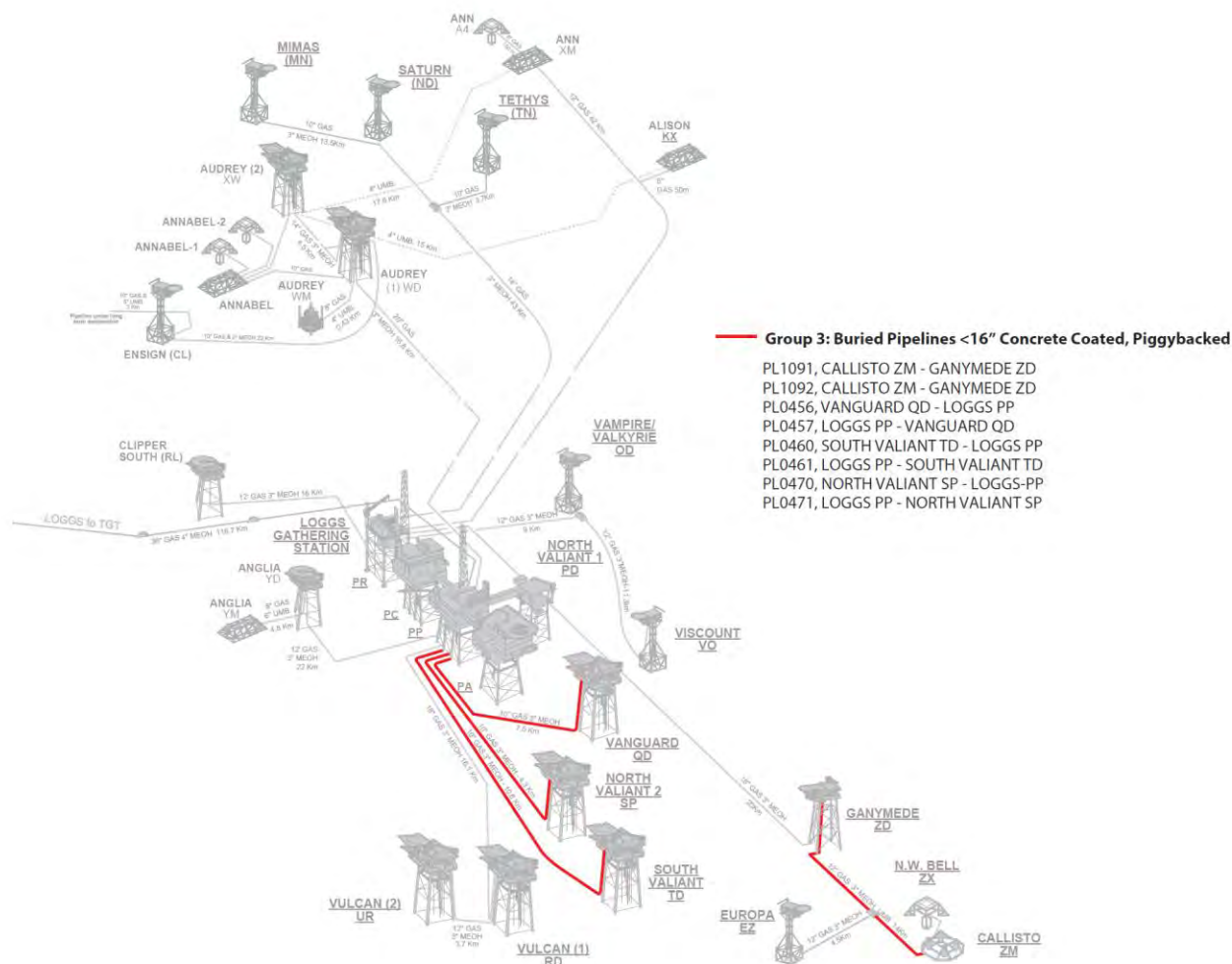
Figure 6-9: LOGGS Area (LDP2 – 5) Group 3c
