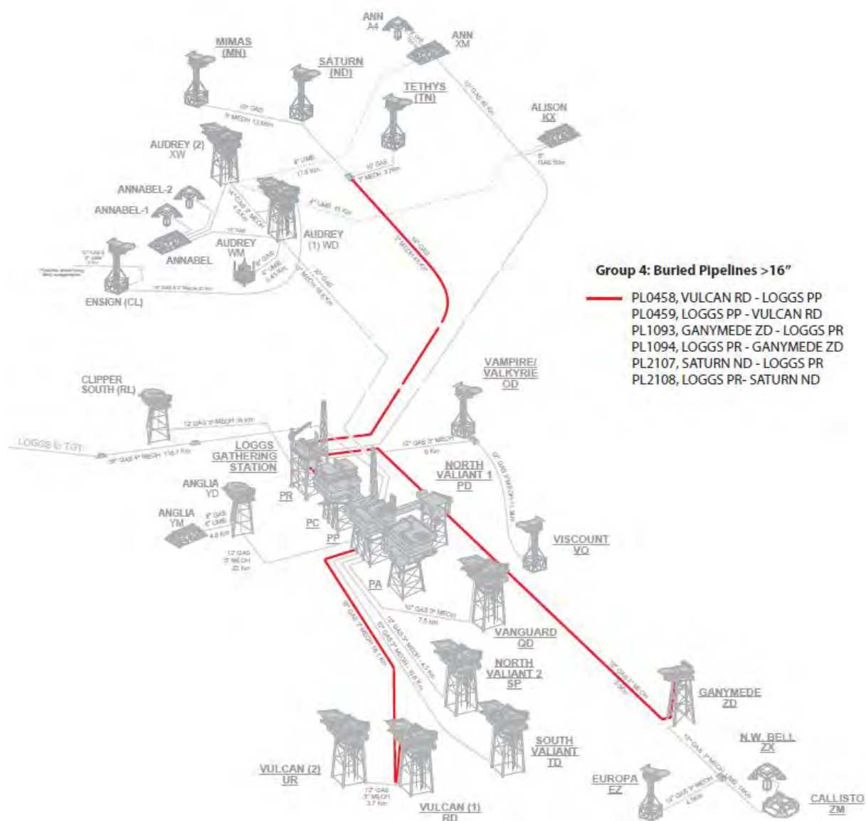
Figure 6-11: LOGGS Area (LDP2 – 5) Group 4
