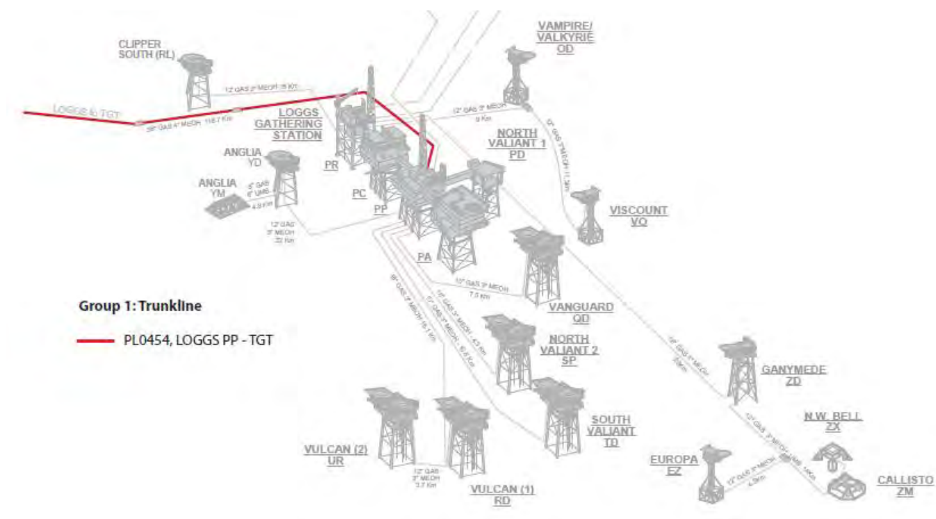
Figure 6-1: LOGGS Area (LDP2 – 5) Group 1
