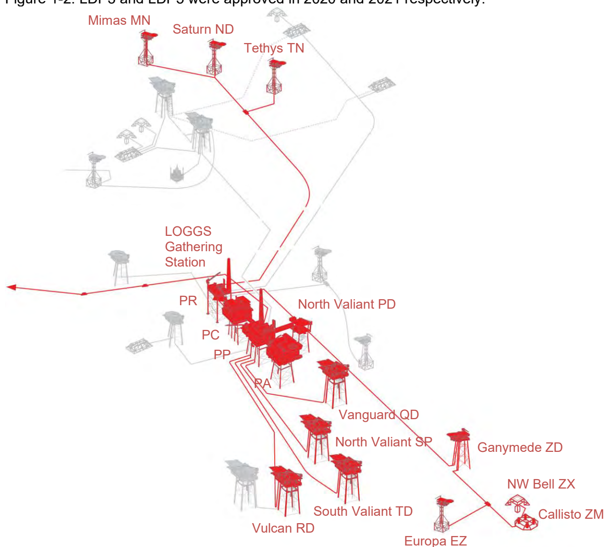
Figure 1-2: Chrysaor LDP2, LDP3, LDP4, LDP5 Decommissioning Programmes Assets in the LOGGS Area
