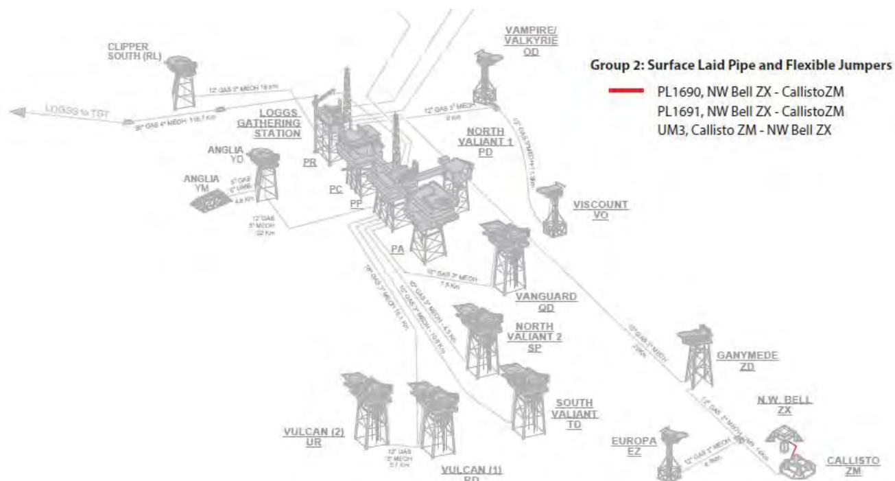
Figure 6-3: LOGGS Area (LDP2 – 5) Group 2
