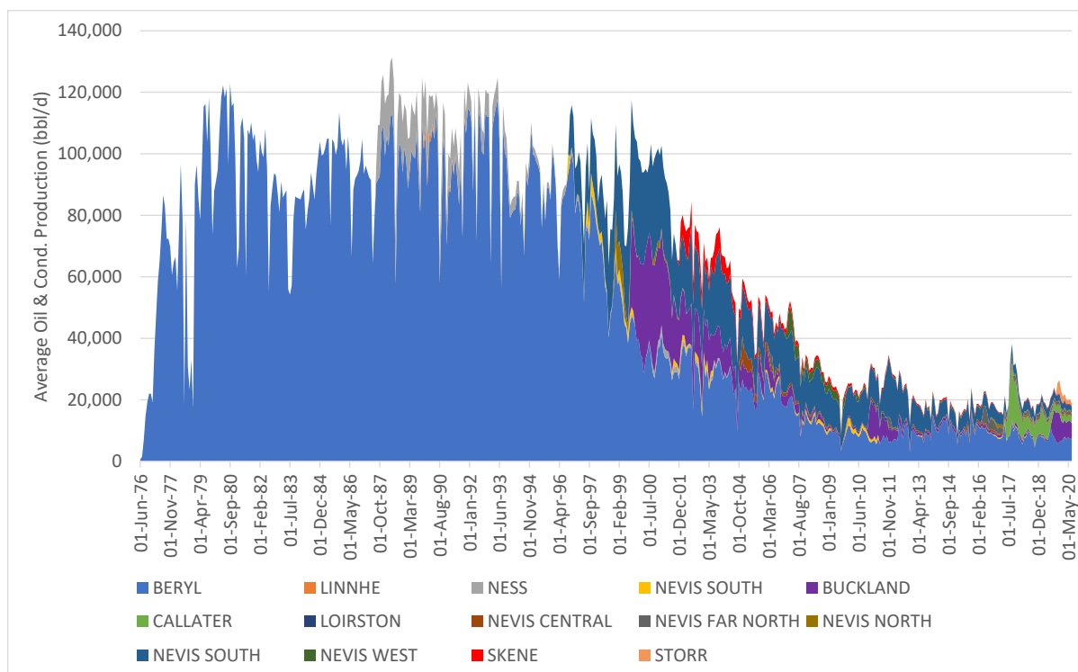
Figure 3-11: Beryl Area oil and condensate production history by field
